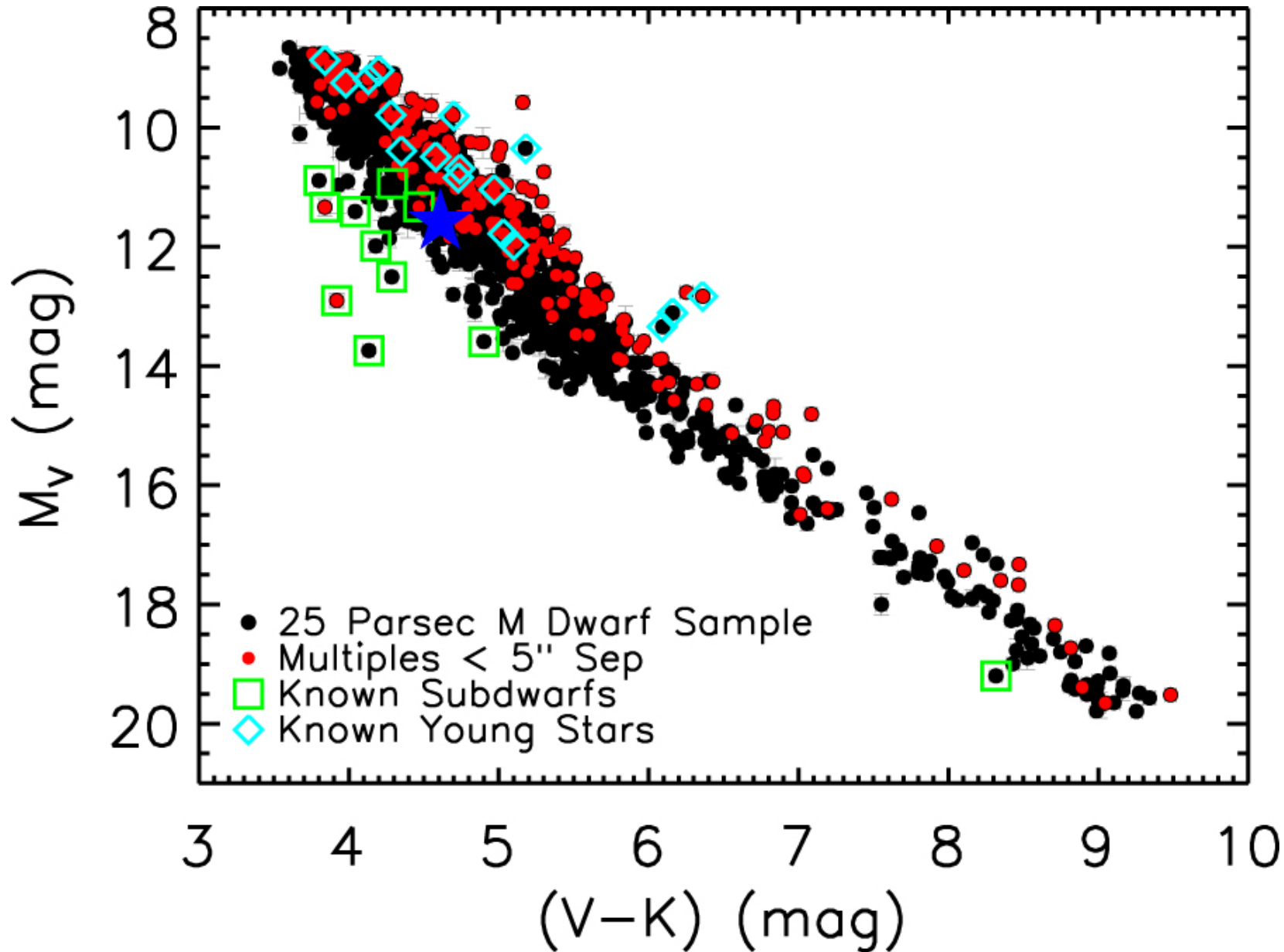
Figure 16. from The L 98-59 System: Three Transiting, Terrestrial-size Planets Orbiting a Nearby M Dwarf null 2019 AJ 158 32 doi:10.3847/1538-3881/ab2459 https://dx.doi.org/10.3847/1538-3881/ab2459 © 2019. The American Astronomical Society. All rights reserved.
