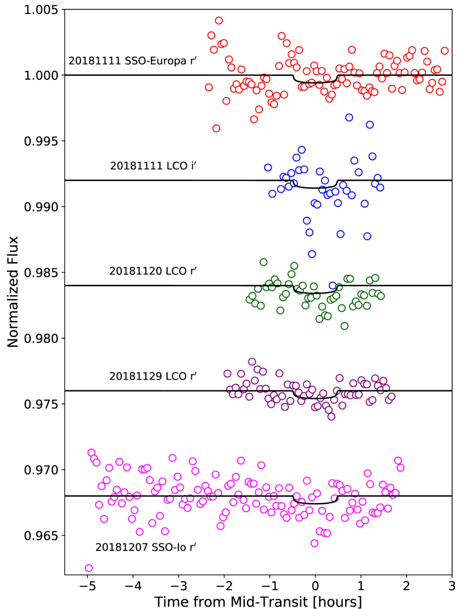
Figure 15. from The L 98-59 System: Three Transiting, Terrestrial-size Planets Orbiting a Nearby M Dwarf null 2019 AJ 158 32 doi:10.3847/1538-3881/ab2459 https://dx.doi.org/10.3847/1538-3881/ab2459 © 2019. The American Astronomical Society. All rights reserved.
