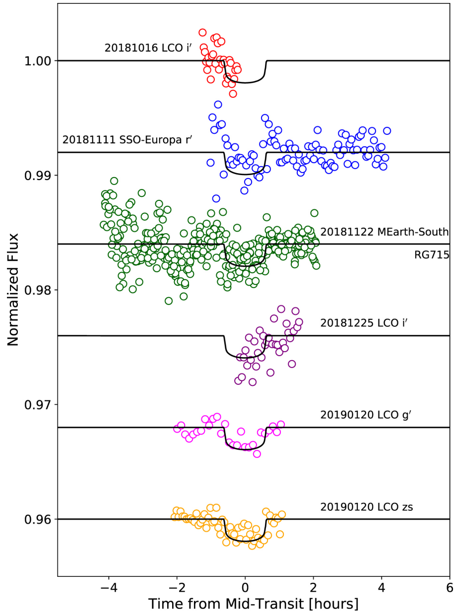
Figure 13. from The L 98-59 System: Three Transiting, Terrestrial-size Planets Orbiting a Nearby M Dwarf null 2019 AJ 158 32 doi:10.3847/1538-3881/ab2459 https://dx.doi.org/10.3847/1538-3881/ab2459 © 2019. The American Astronomical Society. All rights reserved.
