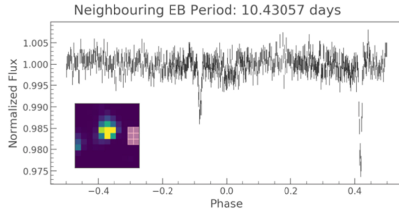
Figure 12. from The L 98-59 System: Three Transiting, Terrestrial-size Planets Orbiting a Nearby M Dwarf null 2019 AJ 158 32 doi:10.3847/1538-3881/ab2459 https://dx.doi.org/10.3847/1538-3881/ab2459 © 2019. The American Astronomical Society. All rights reserved.
