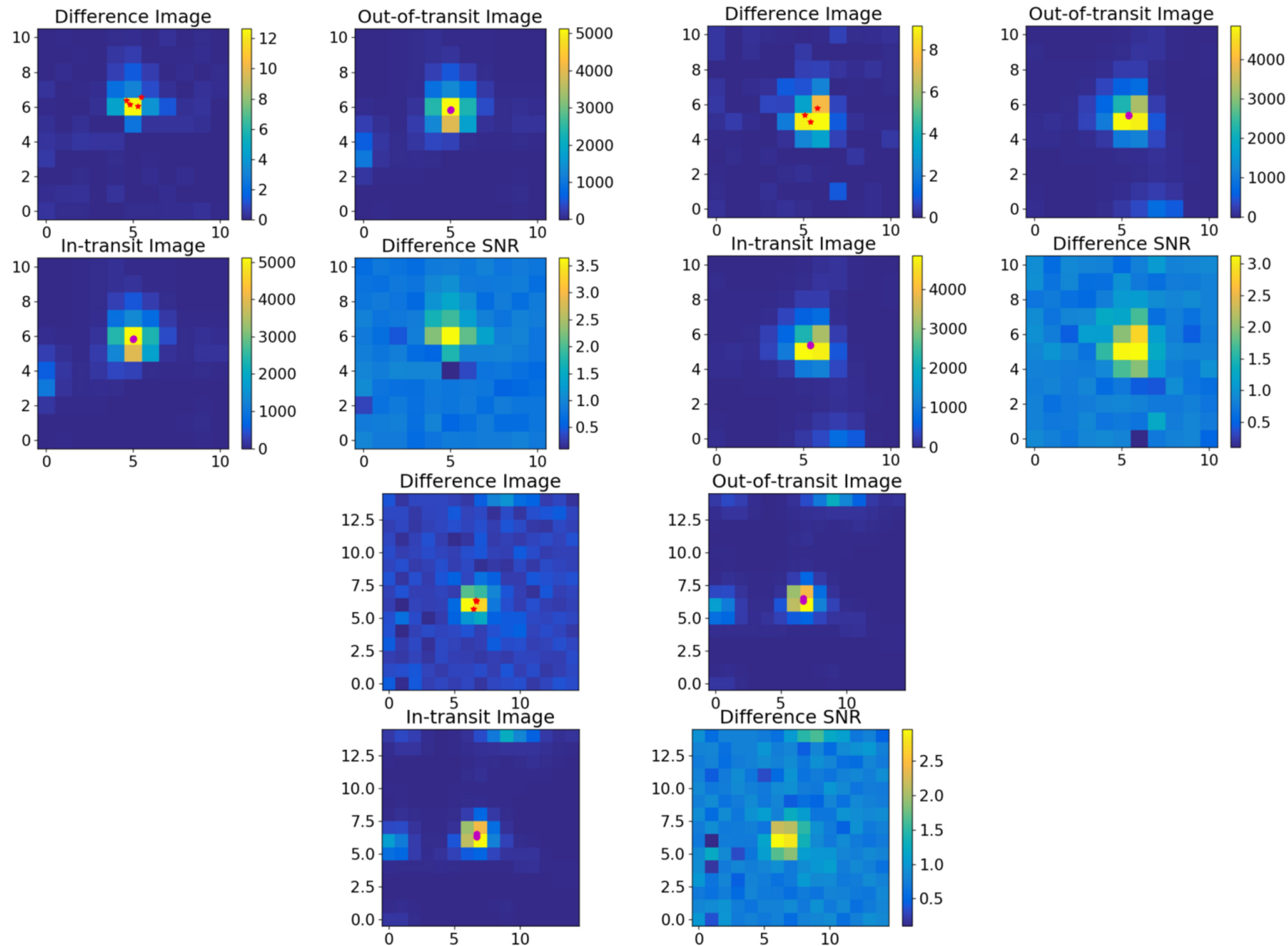
Figure 10. from The L 98-59 System: Three Transiting, Terrestrial-size Planets Orbiting a Nearby M Dwarf null 2019 AJ 158 32 doi:10.3847/1538-3881/ab2459 https://dx.doi.org/10.3847/1538-3881/ab2459 © 2019. The American Astronomical Society. All rights reserved.
