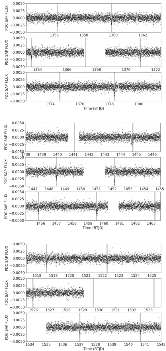
Figure 1. from The L 98-59 System: Three Transiting, Terrestrial-size Planets Orbiting a Nearby M Dwarf null 2019 AJ 158 32 doi:10.3847/1538-3881/ab2459 https://dx.doi.org/10.3847/1538-3881/ab2459 © 2019. The American Astronomical Society. All rights reserved.
