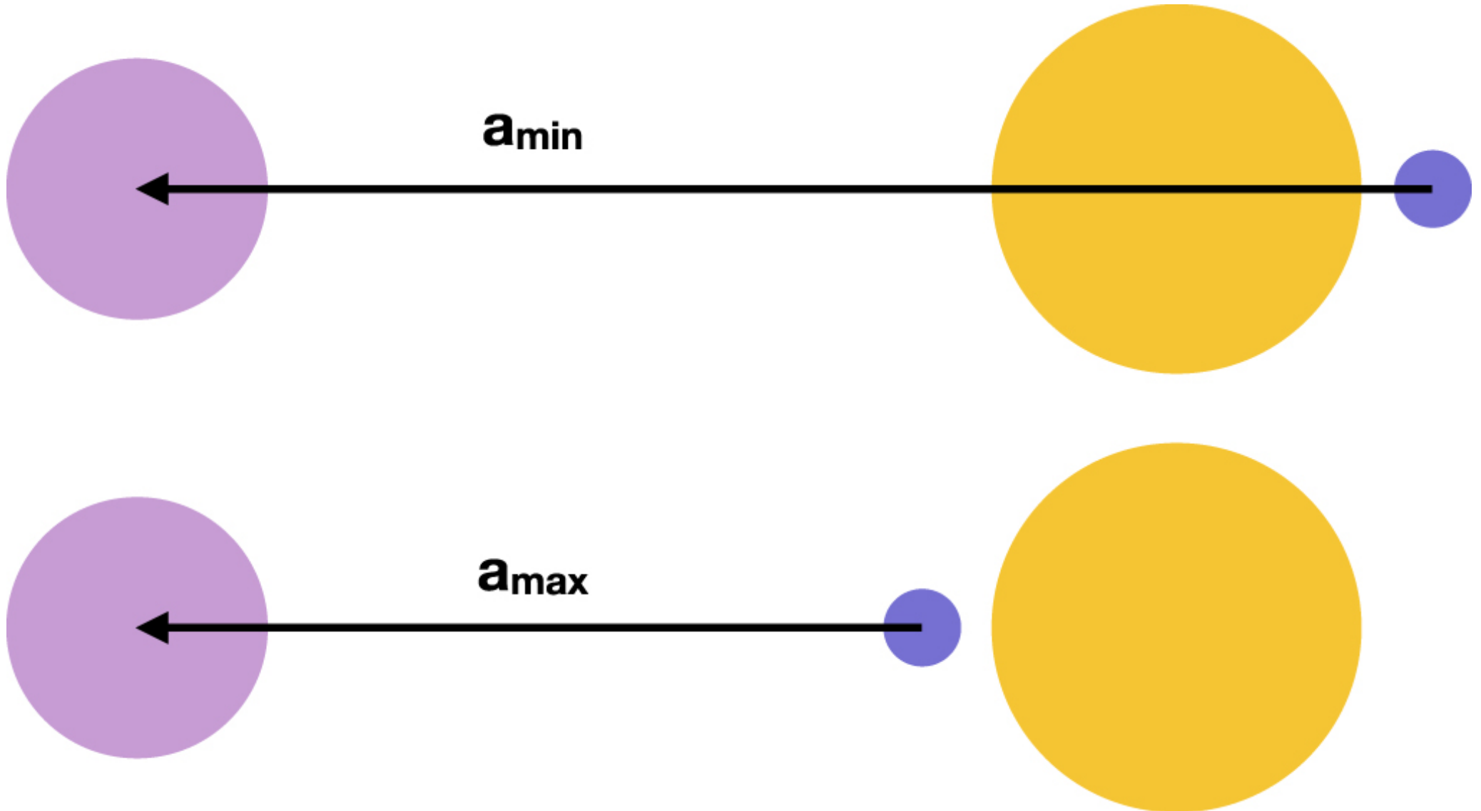
Figure 9. from The Case for a Large-scale Occultation Network null 2019 AJ 158 19 doi:10.3847/1538-3881/ab21df https://dx.doi.org/10.3847/1538-3881/ab21df © 2019. The American Astronomical Society. All rights reserved.
