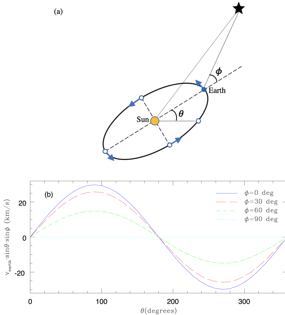
Figure 7. from Optimizing Ground-based Observations of O 2 in Earth Analogs null 2019 AJ 158 24 doi:10.3847/1538-3881/ab21d7 https://dx.doi.org/10.3847/1538-3881/ab21d7 © 2019. The American Astronomical Society. All rights reserved.
