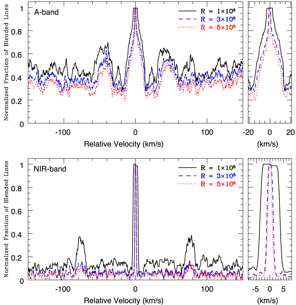
Figure 6. from Optimizing Ground-based Observations of O 2 in Earth Analogs null 2019 AJ 158 24 doi:10.3847/1538-3881/ab21d7 http://dx.doi.org/10.3847/1538-3881/ab21d7 © 2019. The American Astronomical Society. All rights reserved.
