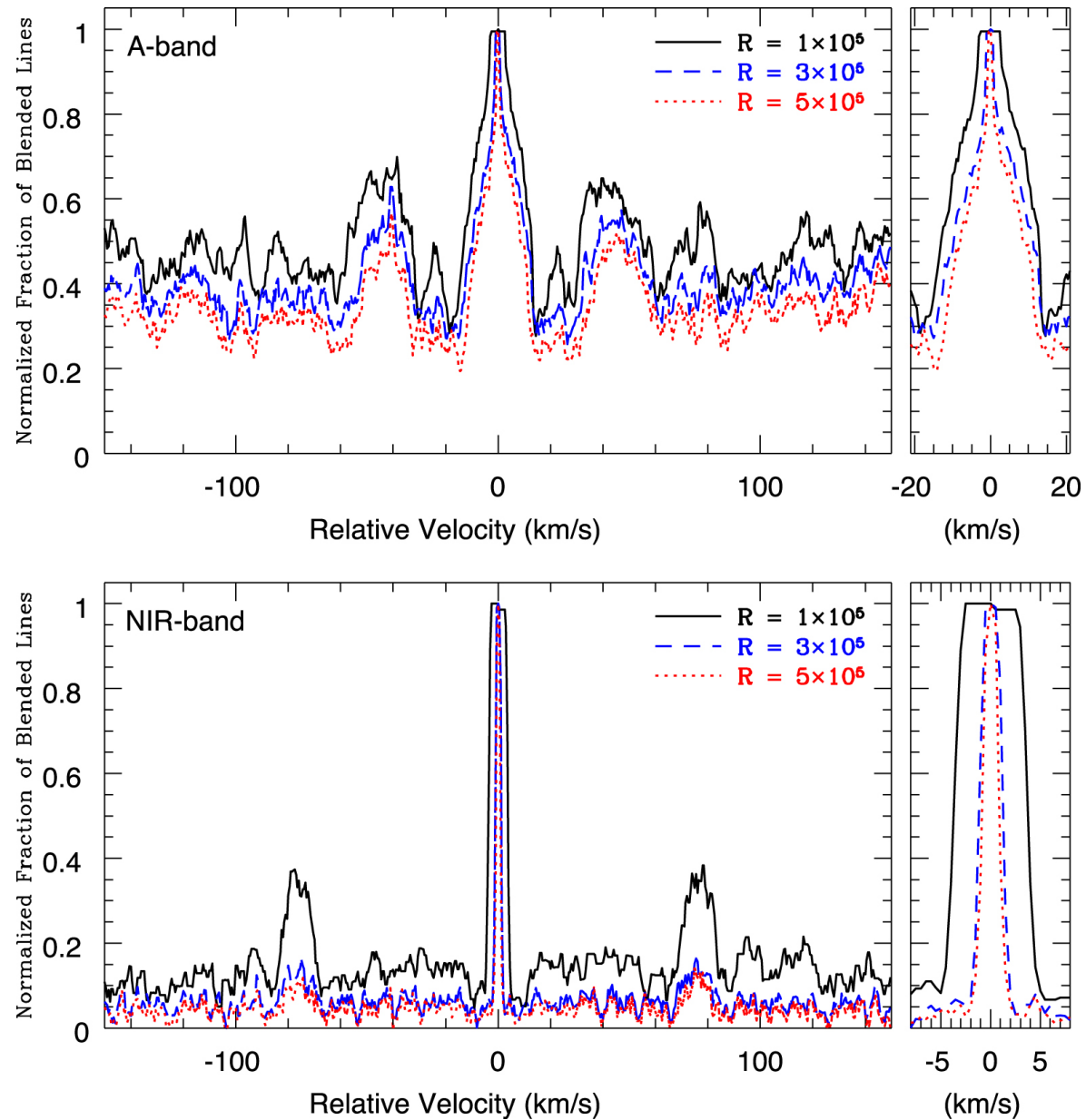
Figure 6. from Optimizing Ground-based Observations of O 2 in Earth Analogs null 2019 AJ 158 24 doi:10.3847/1538-3881/ab21d7 https://dx.doi.org/10.3847/1538-3881/ab21d7 © 2019. The American Astronomical Society. All rights reserved.
