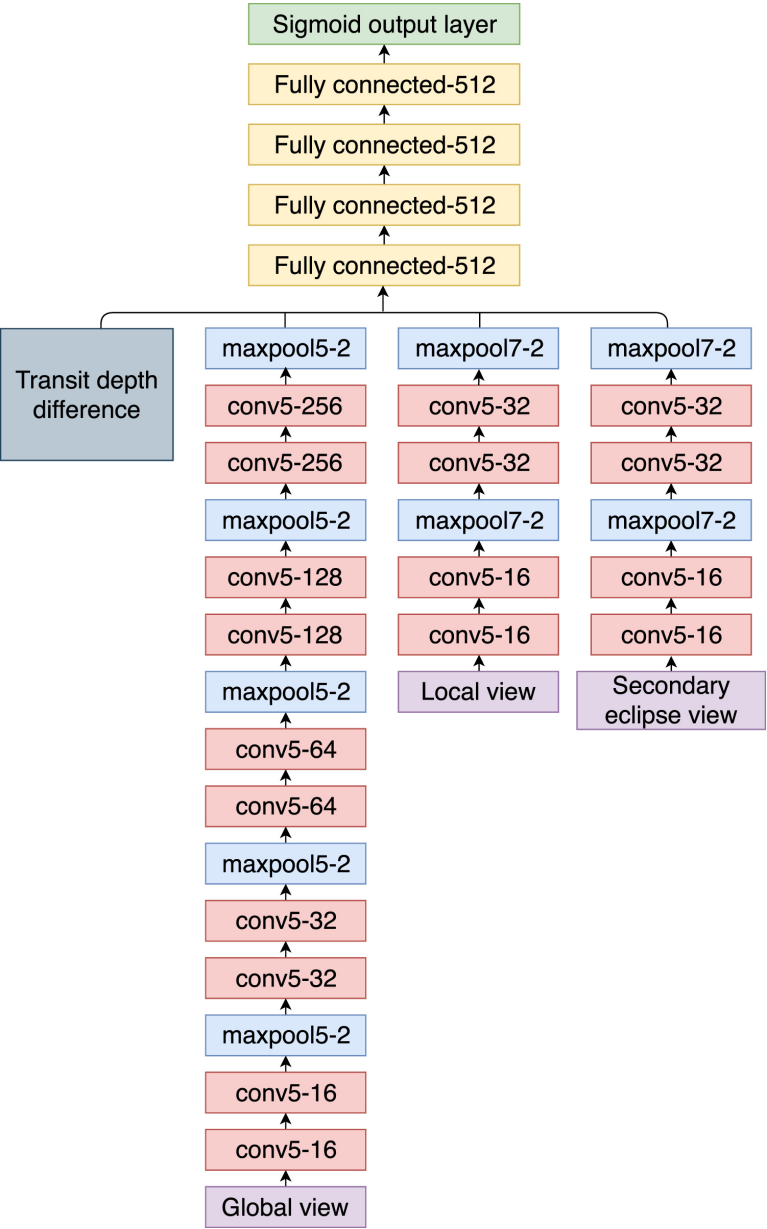
Figure 3. from Identifying Exoplanets with Deep Learning. III. Automated Triage and Vetting of TESS Candidates null 2019 AJ 158 25 doi:10.3847/1538-3881/ab21d6 https://dx.doi.org/10.3847/1538-3881/ab21d6 © 2019. The American Astronomical Society. All rights reserved.
