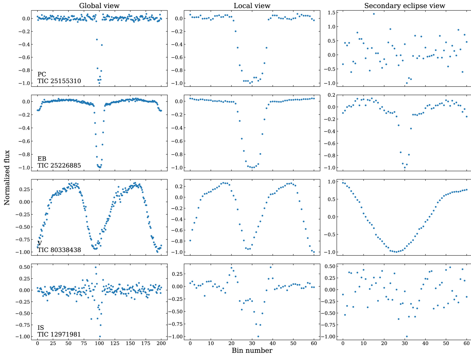
Figure 1. from Identifying Exoplanets with Deep Learning. III. Automated Triage and Vetting of TESS Candidates null 2019 AJ 158 25 doi:10.3847/1538-3881/ab21d6 https://dx.doi.org/10.3847/1538-3881/ab21d6 © 2019. The American Astronomical Society. All rights reserved.
