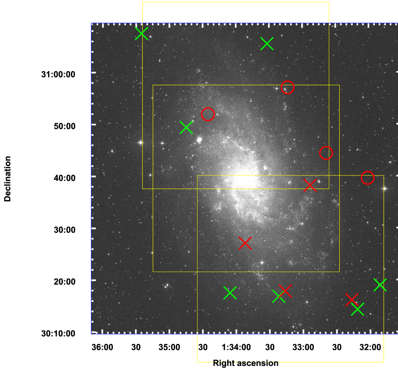
Figure 5. from The Discovery of Quasi-stellar Objects behind M31 and M33 null 2019 AJ 157 227 doi:10.3847/1538-3881/ab1aa1 https://dx.doi.org/10.3847/1538-3881/ab1aa1 © 2019. The American Astronomical Society. All rights reserved.
