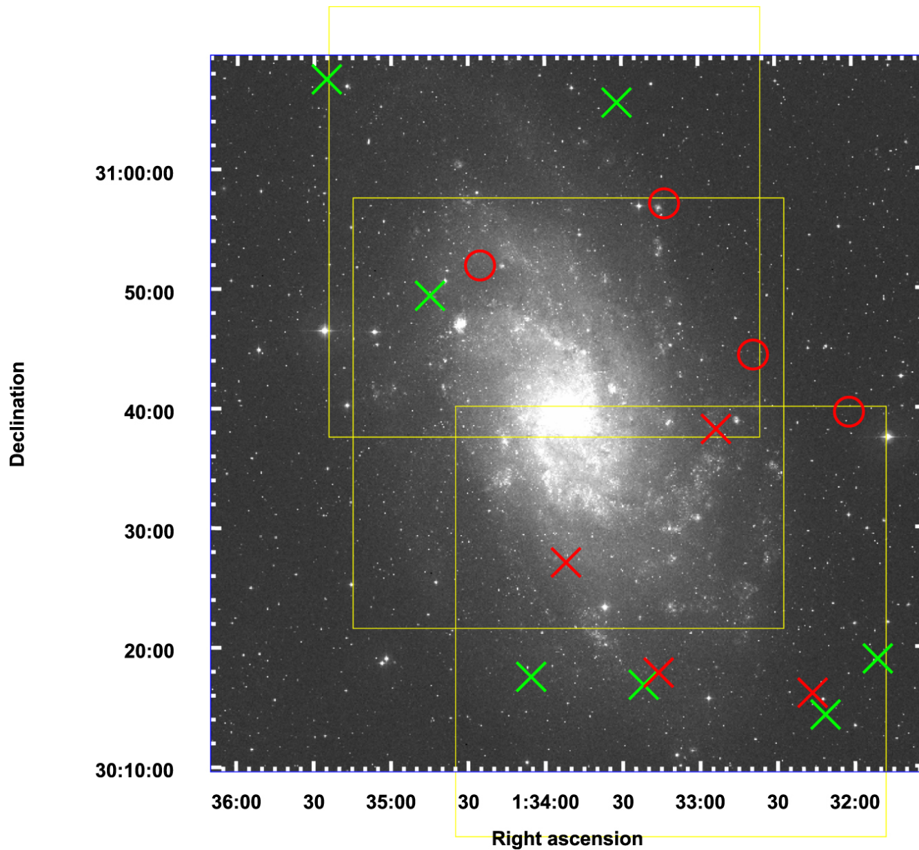
Figure 5. from The Discovery of Quasi-stellar Objects behind M31 and M33 null 2019 AJ 157 227 doi:10.3847/1538-3881/ab1aa1 http://dx.doi.org/10.3847/1538-3881/ab1aa1 © 2019. The American Astronomical Society. All rights reserved.
