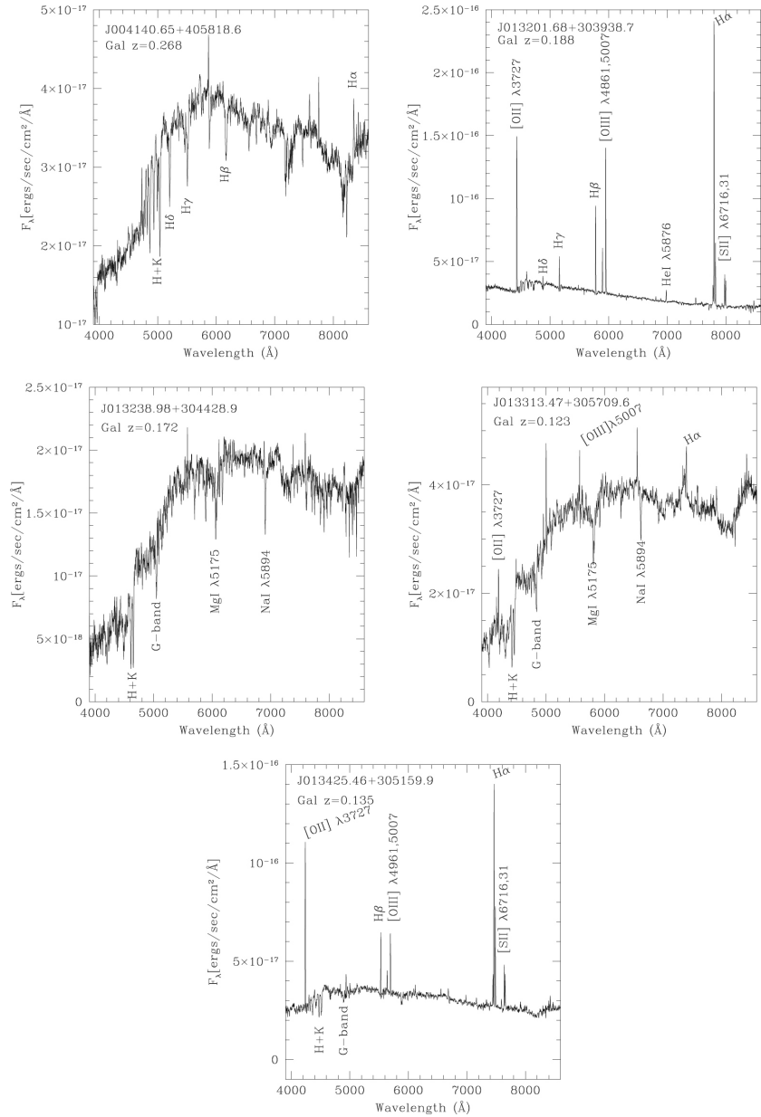
Figure 2. from The Discovery of Quasi-stellar Objects behind M31 and M33 null 2019 AJ 157 227 doi:10.3847/1538-3881/ab1aa1 http://dx.doi.org/10.3847/1538-3881/ab1aa1 © 2019. The American Astronomical Society. All rights reserved.
