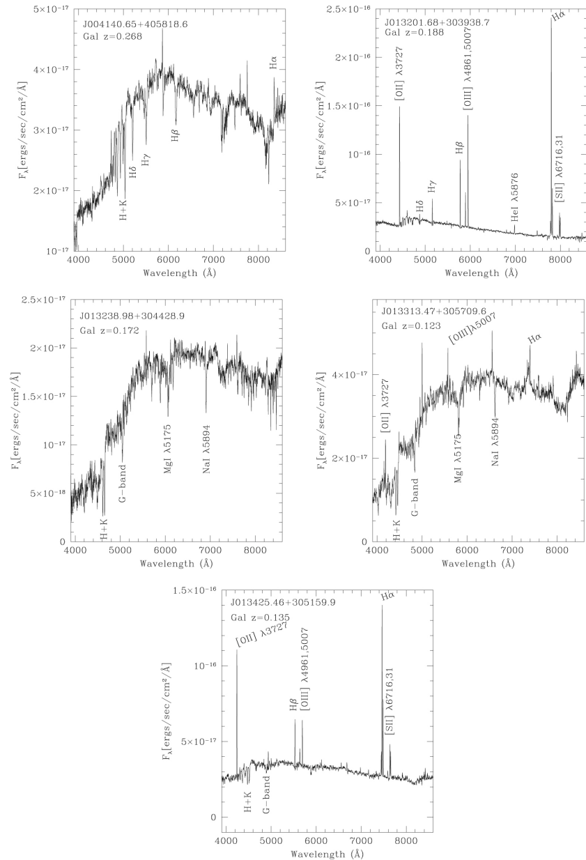
Figure 2. from The Discovery of Quasi-stellar Objects behind M31 and M33 null 2019 AJ 157 227 doi:10.3847/1538-3881/ab1aa1 https://dx.doi.org/10.3847/1538-3881/ab1aa1 © 2019. The American Astronomical Society. All rights reserved.
