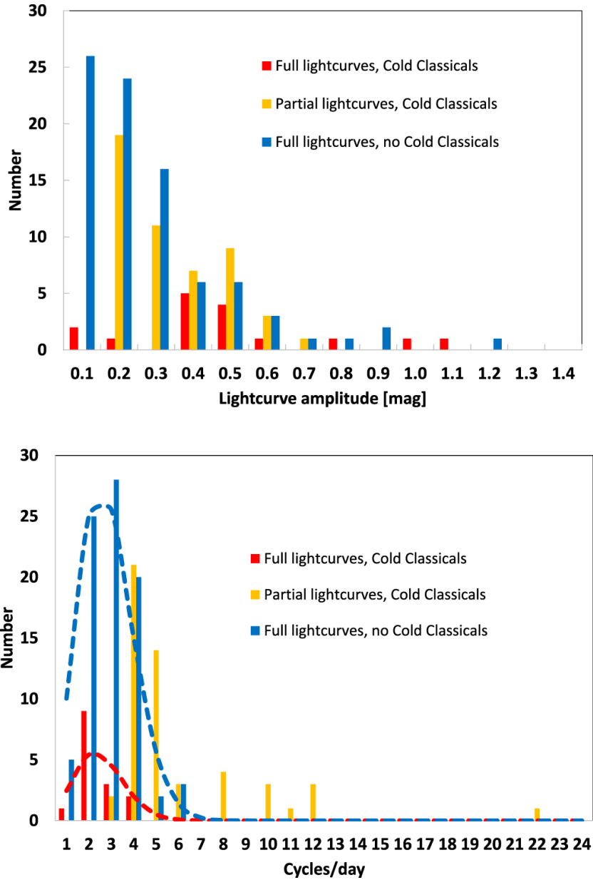
Figure 7. from Light Curves and Rotational Properties of the Pristine Cold Classical Kuiper Belt Objects null 2019 AJ 157 228 doi:10.3847/1538-3881/ab18a9 https://dx.doi.org/10.3847/1538-3881/ab18a9 © 2019. The American Astronomical Society. All rights reserved.
