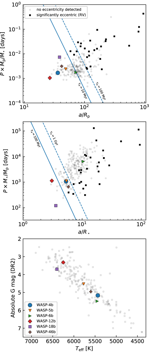
Figure 5. from WASP-4b Arrived Early for the TESS Mission null 2019 AJ 157 217 doi:10.3847/1538-3881/ab189f https://dx.doi.org/10.3847/1538-3881/ab189f © 2019. The American Astronomical Society. All rights reserved.
