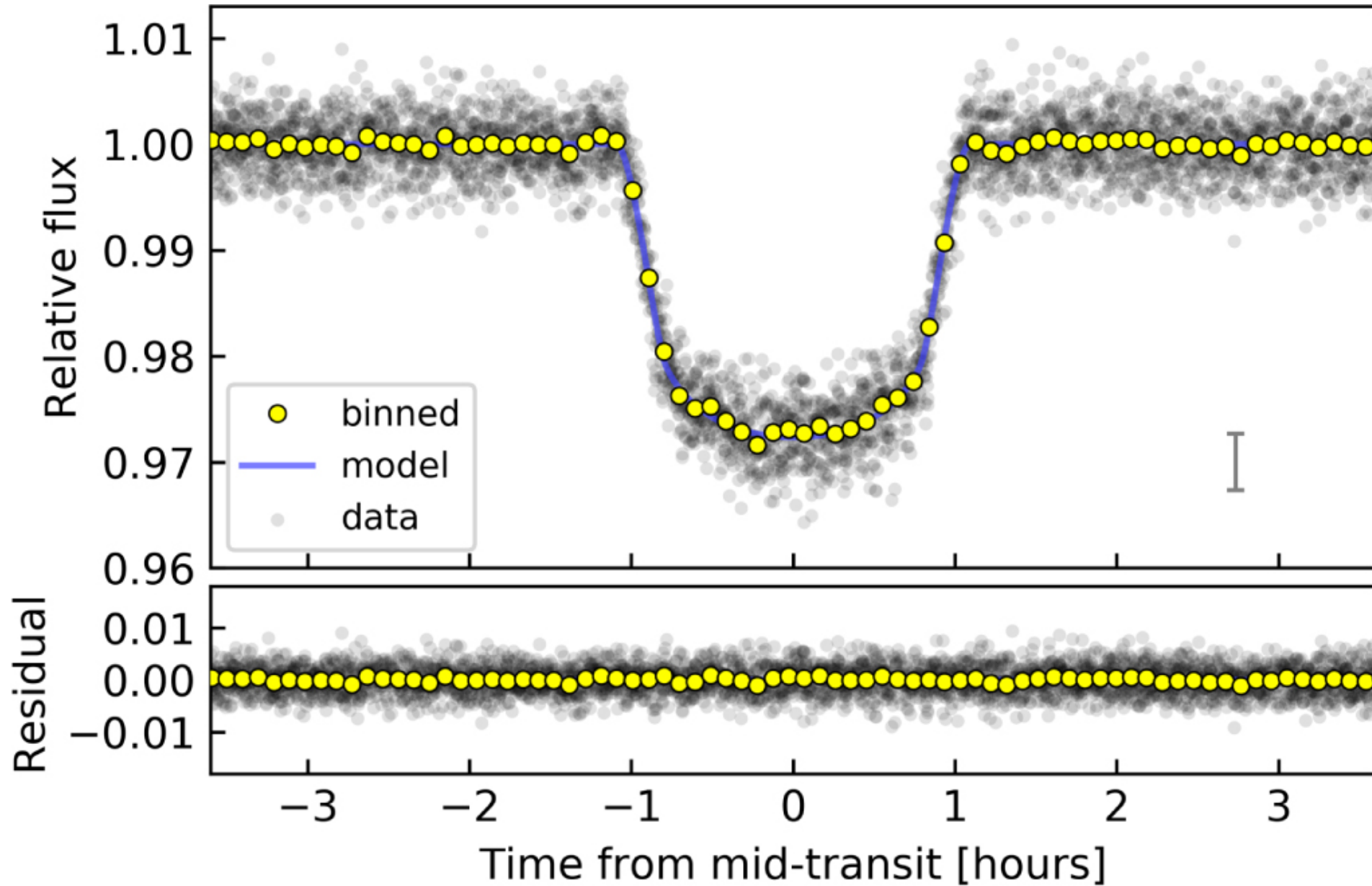
Figure 2. from WASP-4b Arrived Early for the TESS Mission null 2019 AJ 157 217 doi:10.3847/1538-3881/ab189f https://dx.doi.org/10.3847/1538-3881/ab189f © 2019. The American Astronomical Society. All rights reserved.
