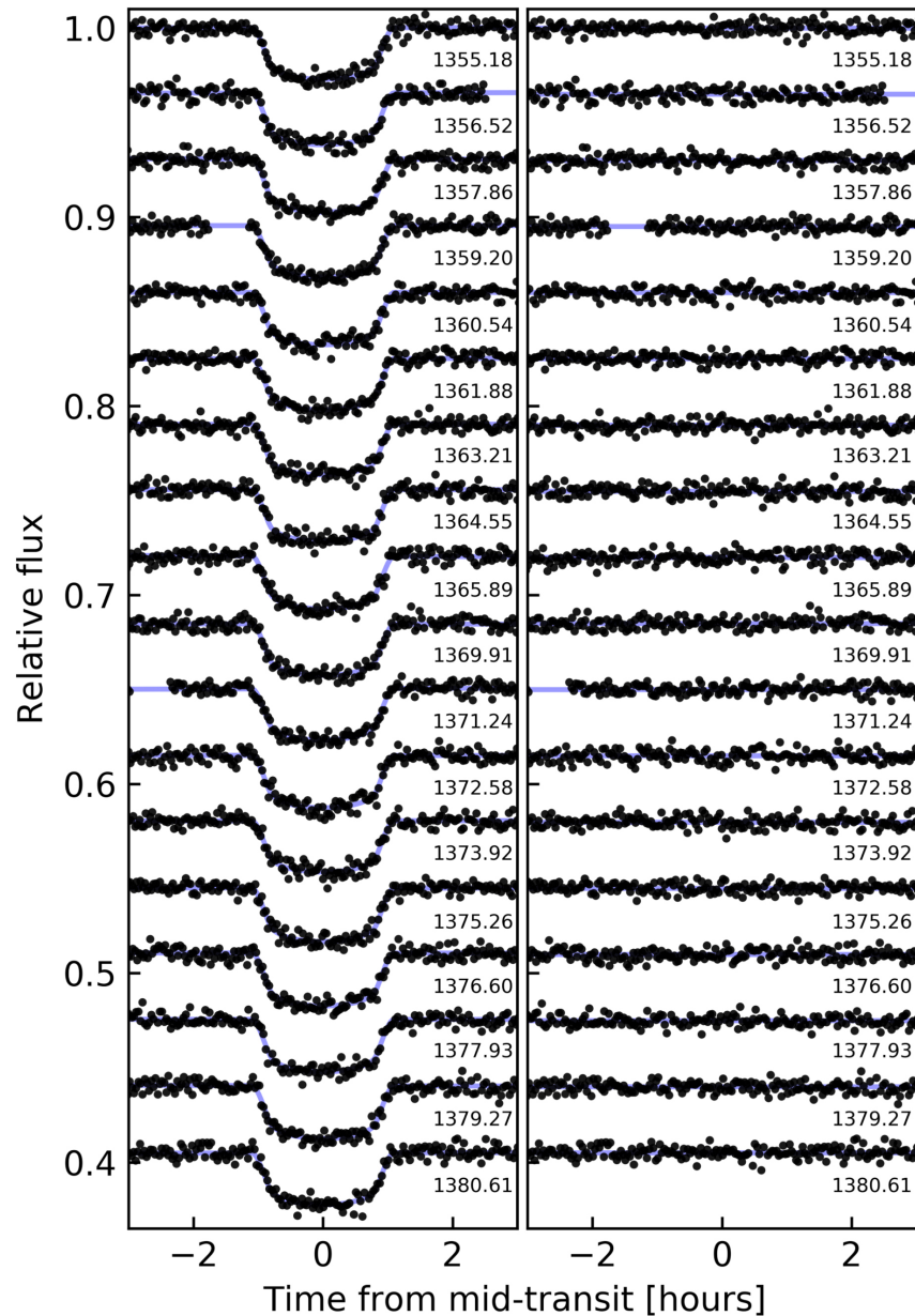
Figure 1. from WASP-4b Arrived Early for the TESS Mission null 2019 AJ 157 217 doi:10.3847/1538-3881/ab189f https://dx.doi.org/10.3847/1538-3881/ab189f © 2019. The American Astronomical Society. All rights reserved.
