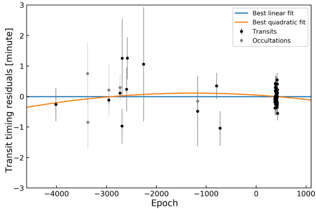
Figure 5. from TESS Full Orbital Phase Curve of the WASP-18b System null 2019 AJ 157 178 doi:10.3847/1538-3881/ab0f96 https://dx.doi.org/10.3847/1538-3881/ab0f96 © 2019. The American Astronomical Society. All rights reserved.
