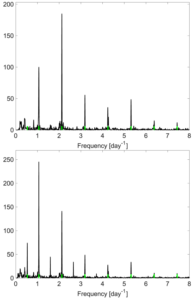
Figure 4. from TESS Full Orbital Phase Curve of the WASP-18b System null 2019 AJ 157 178 doi:10.3847/1538-3881/ab0f96 https://dx.doi.org/10.3847/1538-3881/ab0f96 © 2019. The American Astronomical Society. All rights reserved.
