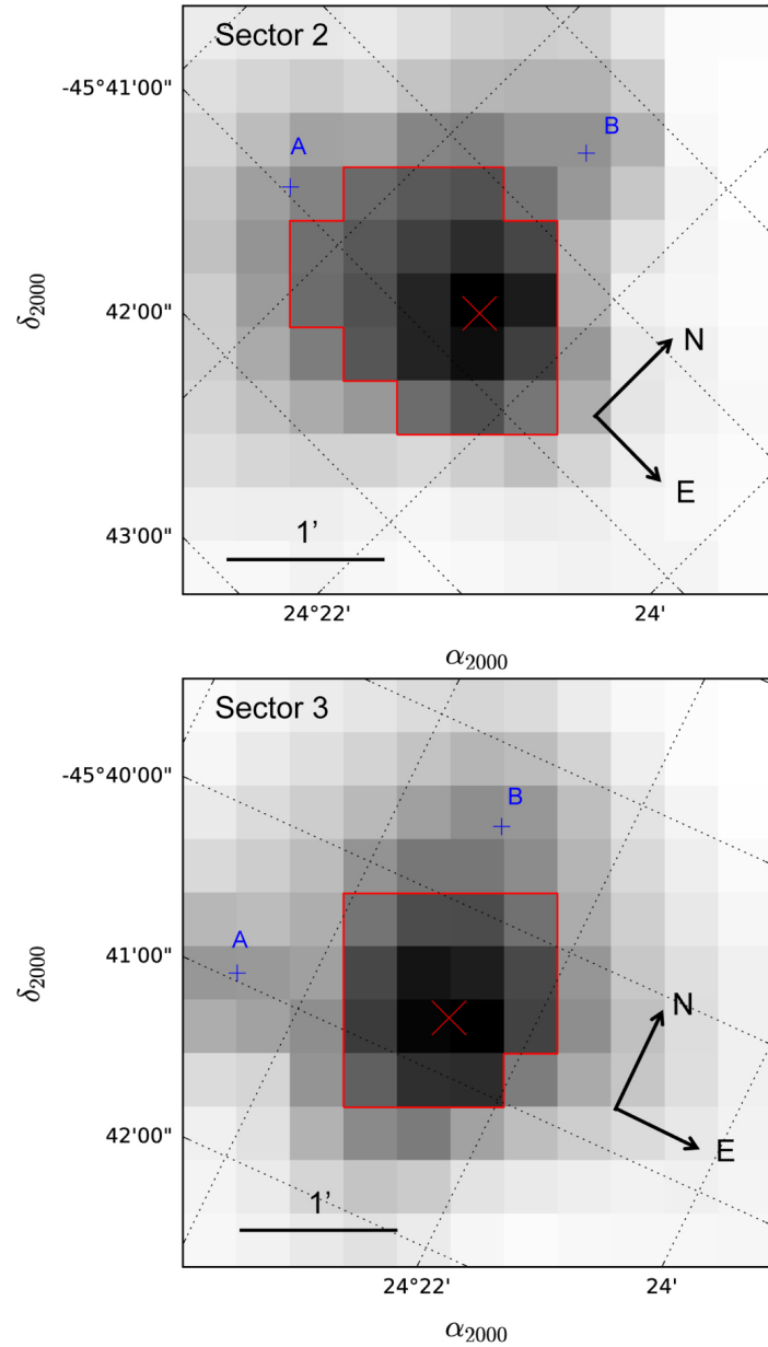
Figure 1. from TESS Full Orbital Phase Curve of the WASP-18b System null 2019 AJ 157 178 doi:10.3847/1538-3881/ab0f96 https://dx.doi.org/10.3847/1538-3881/ab0f96 © 2019. The American Astronomical Society. All rights reserved.
