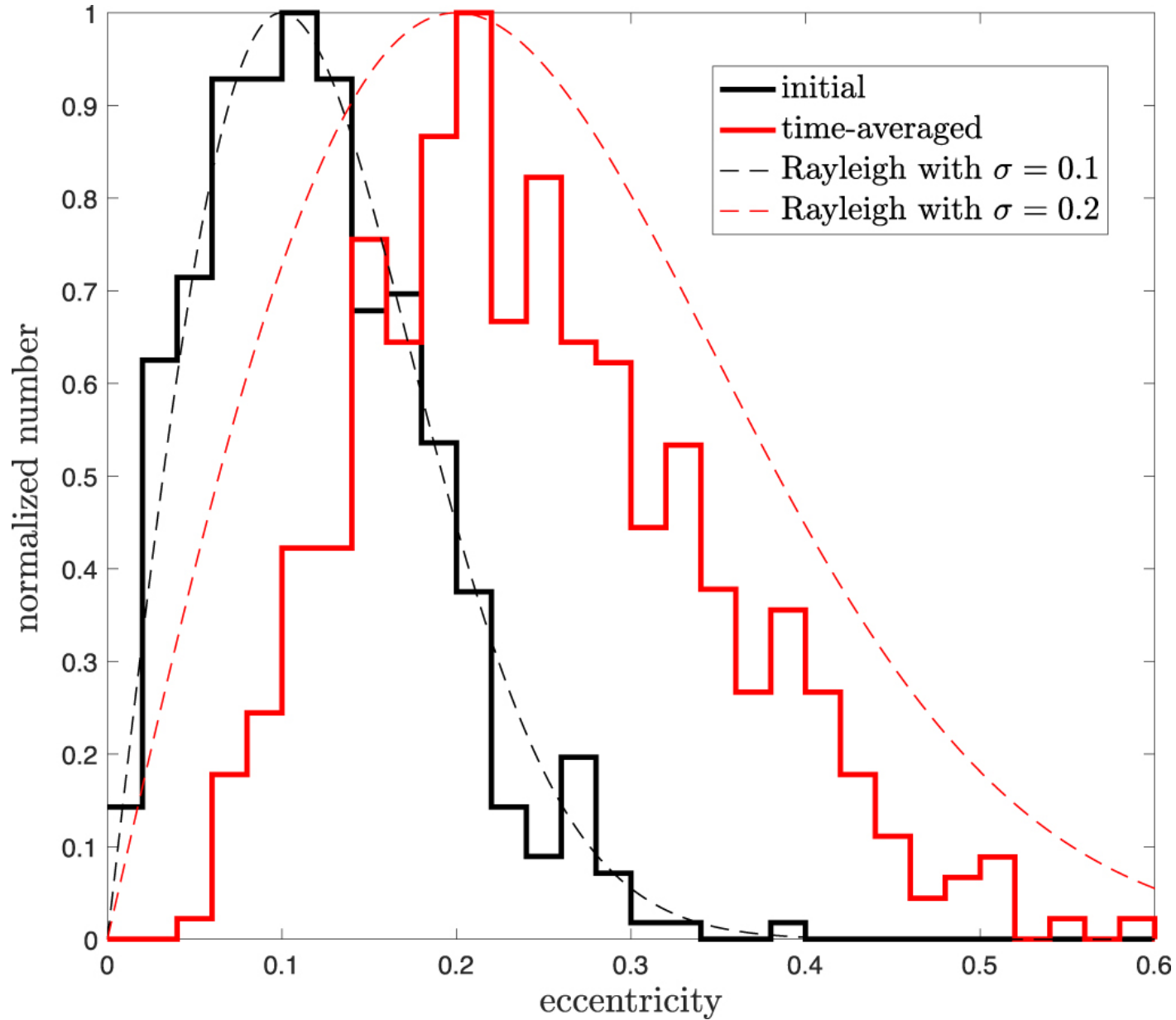
Figure 9. from Ultra-short-period Planets from Secular Chaos null 2019 AJ 157 180 doi:10.3847/1538-3881/ab0e0a https://dx.doi.org/10.3847/1538-3881/ab0e0a © 2019. The American Astronomical Society. All rights reserved.
