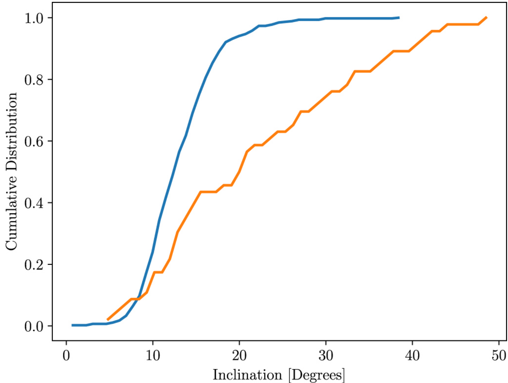
Figure 8. from Ultra-short-period Planets from Secular Chaos null 2019 AJ 157 180 doi:10.3847/1538-3881/ab0e0a https://dx.doi.org/10.3847/1538-3881/ab0e0a © 2019. The American Astronomical Society. All rights reserved.
