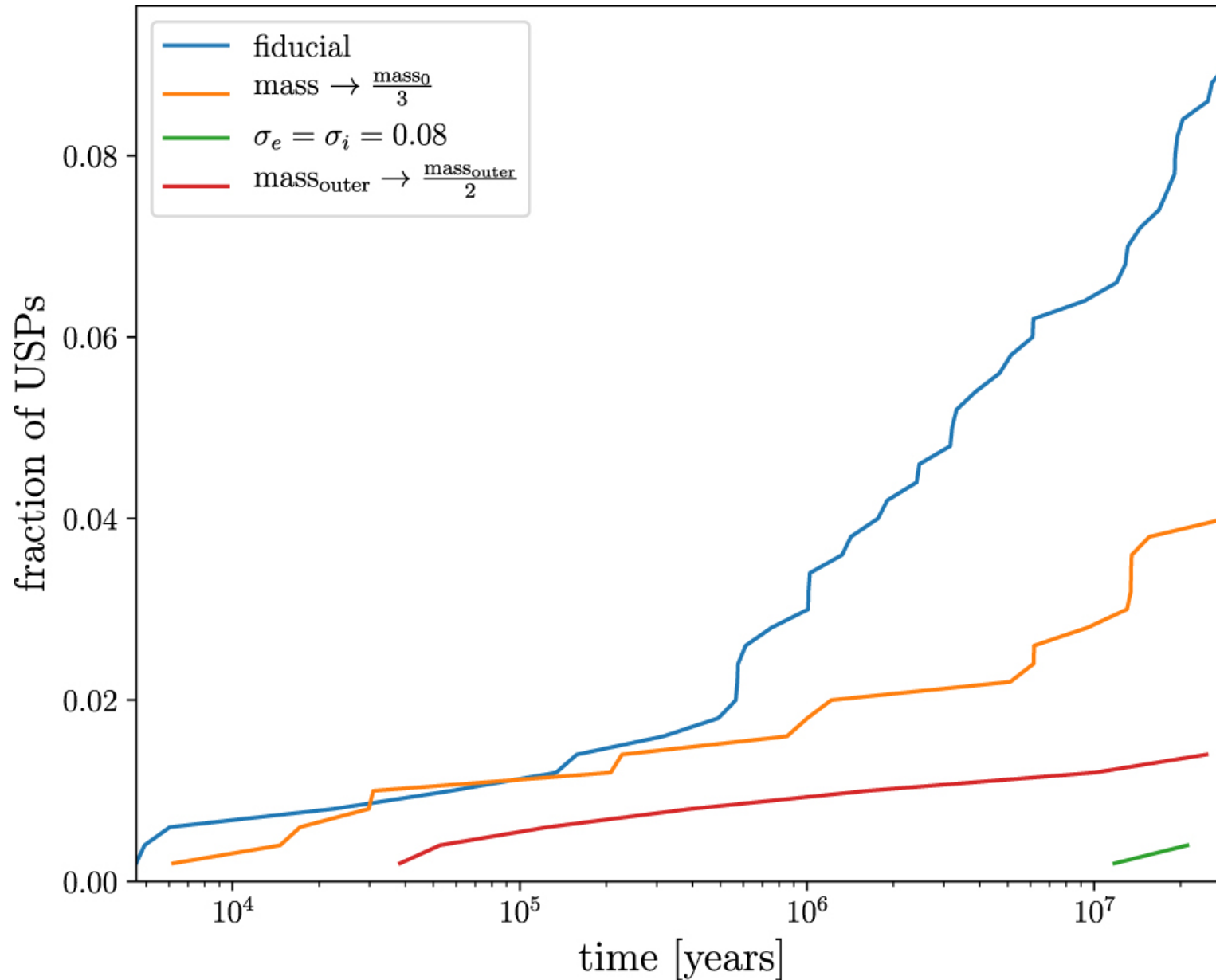
Figure 7. from Ultra-short-period Planets from Secular Chaos null 2019 AJ 157 180 doi:10.3847/1538-3881/ab0e0a https://dx.doi.org/10.3847/1538-3881/ab0e0a © 2019. The American Astronomical Society. All rights reserved.
