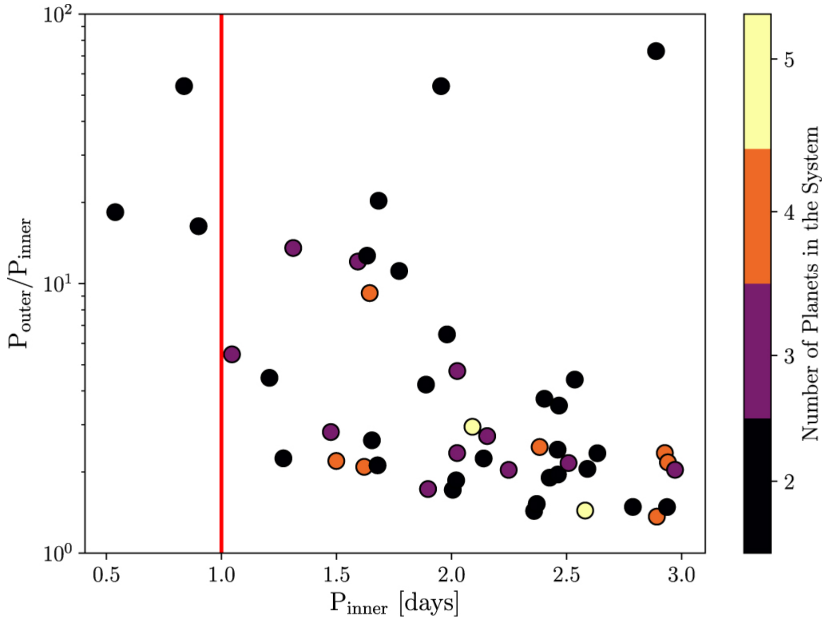
Figure 1. from Ultra-short-period Planets from Secular Chaos null 2019 AJ 157 180 doi:10.3847/1538-3881/ab0e0a https://dx.doi.org/10.3847/1538-3881/ab0e0a © 2019. The American Astronomical Society. All rights reserved.
