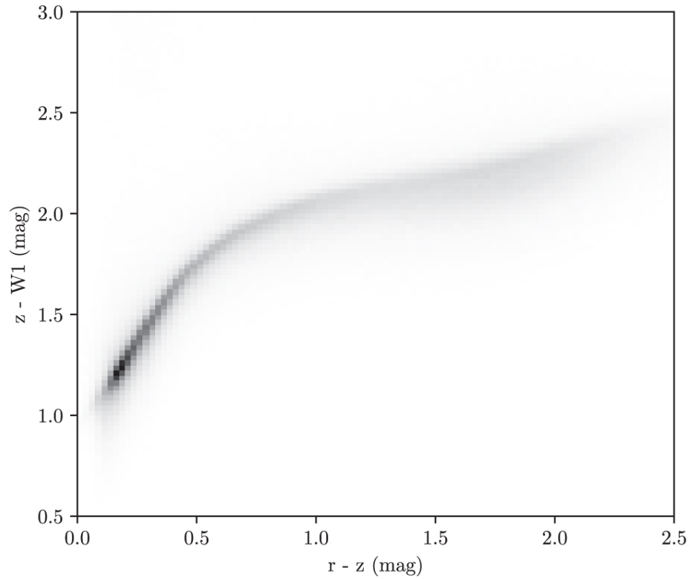
Figure 9. from Overview of the DESI Legacy Imaging Surveys null 2019 AJ 157 168 doi:10.3847/1538-3881/ab089d https://dx.doi.org/10.3847/1538-3881/ab089d © 2019. The American Astronomical Society. All rights reserved.
