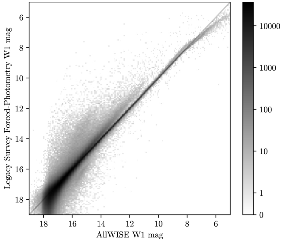
Figure 8. from Overview of the DESI Legacy Imaging Surveys null 2019 AJ 157 168 doi:10.3847/1538-3881/ab089d https://dx.doi.org/10.3847/1538-3881/ab089d © 2019. The American Astronomical Society. All rights reserved.
