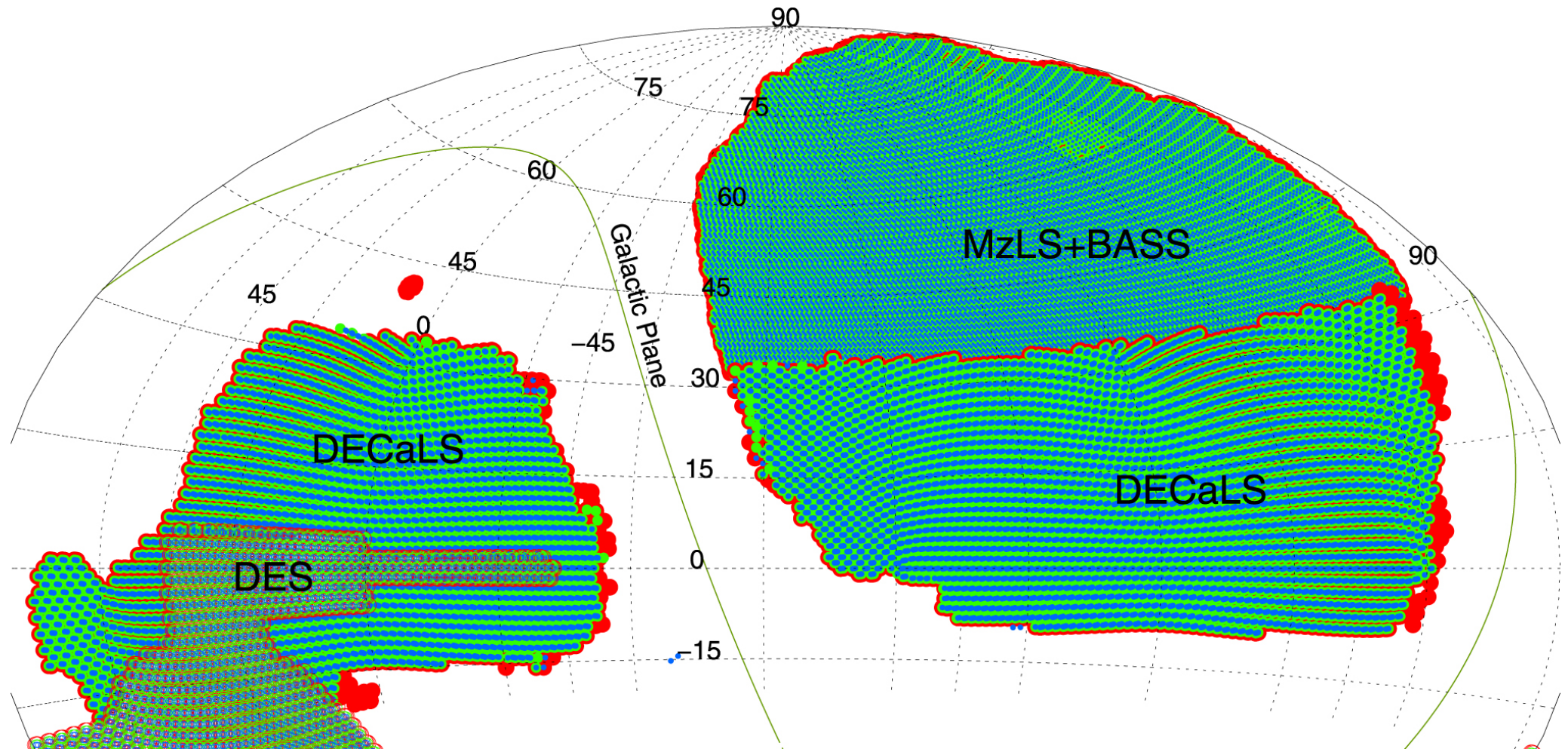
Figure 2. from Overview of the DESI Legacy Imaging Surveys null 2019 AJ 157 168 doi:10.3847/1538-3881/ab089d https://dx.doi.org/10.3847/1538-3881/ab089d © 2019. The American Astronomical Society. All rights reserved.
