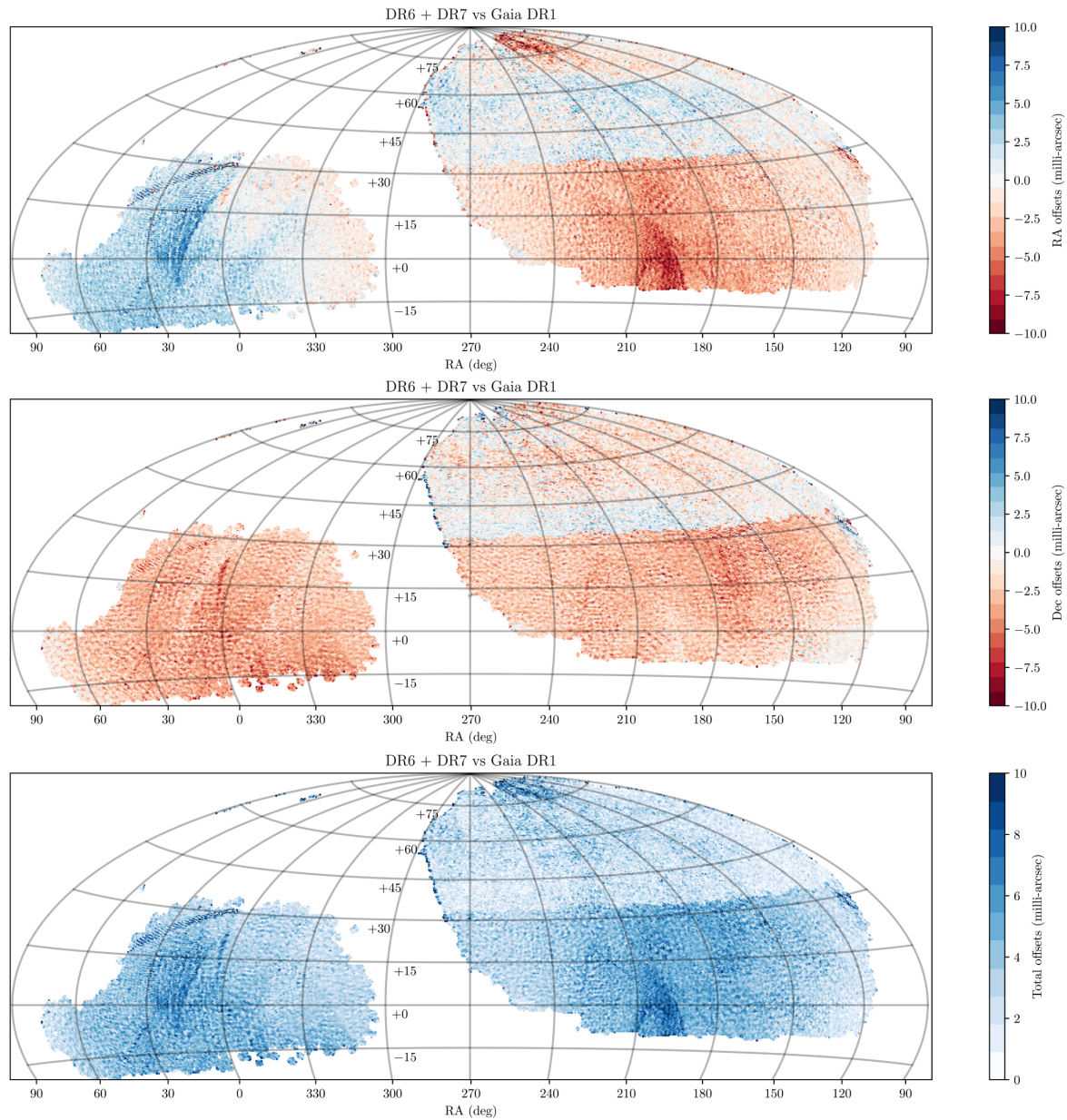
Figure 11. from Overview of the DESI Legacy Imaging Surveys null 2019 AJ 157 168 doi:10.3847/1538-3881/ab089d https://dx.doi.org/10.3847/1538-3881/ab089d © 2019. The American Astronomical Society. All rights reserved.
