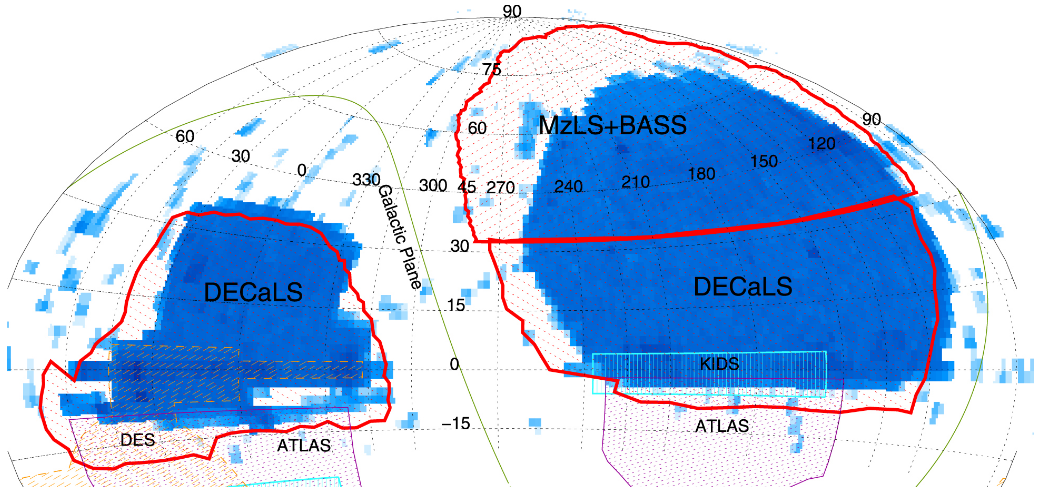
Figure 1. from Overview of the DESI Legacy Imaging Surveys null 2019 AJ 157 168 doi:10.3847/1538-3881/ab089d https://dx.doi.org/10.3847/1538-3881/ab089d © 2019. The American Astronomical Society. All rights reserved.
