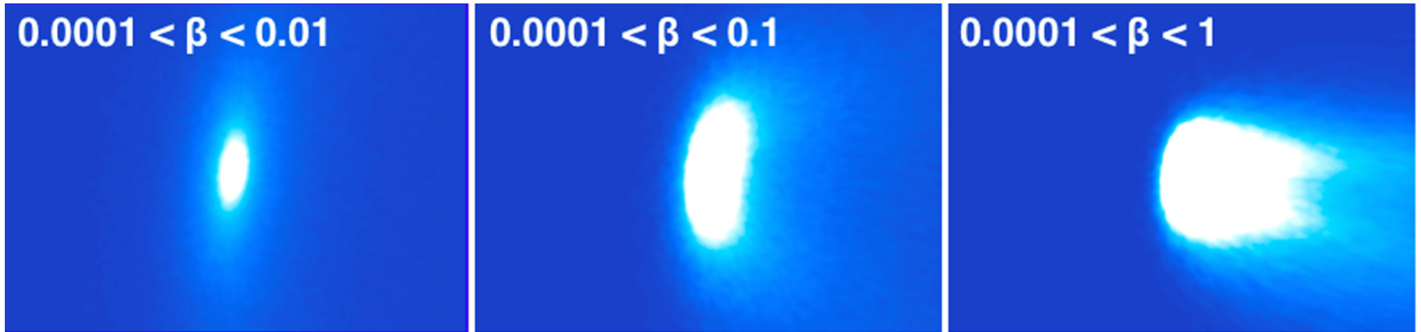
Figure 9. from The Discus Comet: C/2014 B1 (Schwartz) null 2019 AJ 157 103 doi:10.3847/1538-3881/aafe05 https://dx.doi.org/10.3847/1538-3881/aafe05 © 2019. The American Astronomical Society. All rights reserved.
