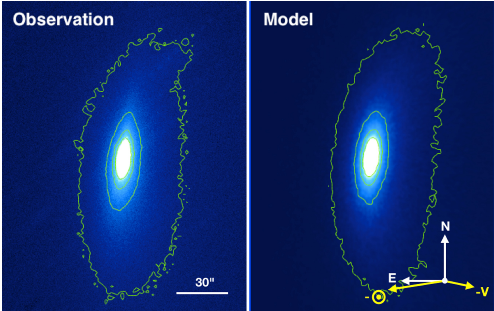
Figure 8. from The Discus Comet: C/2014 B1 (Schwartz) null 2019 AJ 157 103 doi:10.3847/1538-3881/aafe05 https://dx.doi.org/10.3847/1538-3881/aafe05 © 2019. The American Astronomical Society. All rights reserved.
