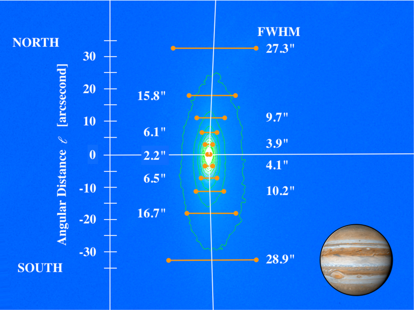
Figure 6. from The Discus Comet: C/2014 B1 (Schwartz) null 2019 AJ 157 103 doi:10.3847/1538-3881/aafe05 https://dx.doi.org/10.3847/1538-3881/aafe05 © 2019. The American Astronomical Society. All rights reserved.
