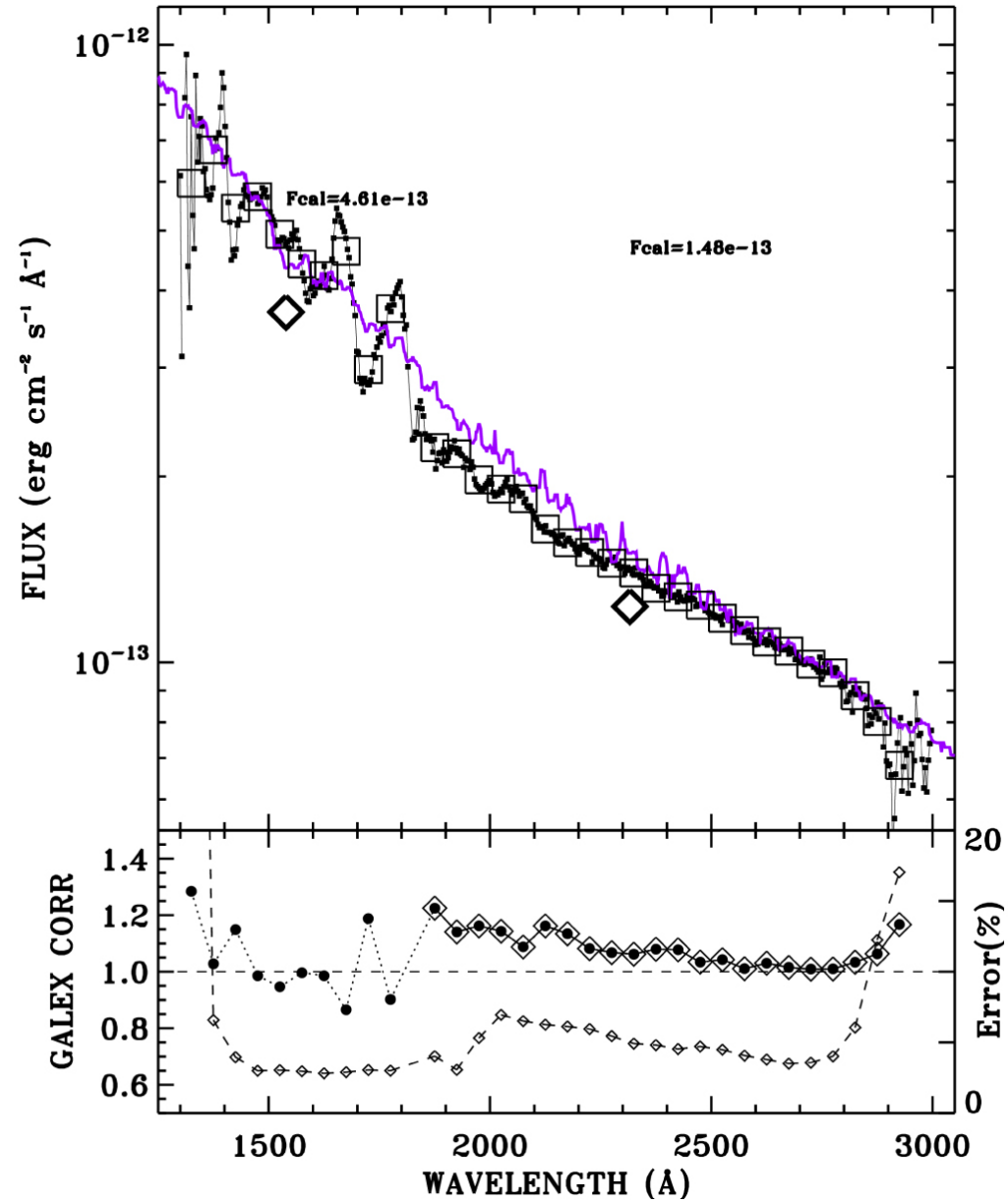
Figure 6. from A Correction for GALEX Spectroscopic UV Flux Distributions from Comparisons with CALSPEC and IUE null 2019 AJ 157 107 doi:10.3847/1538-3881/aafdb8 https://dx.doi.org/10.3847/1538-3881/aafdb8 © 2019. The American Astronomical Society. All rights reserved.
