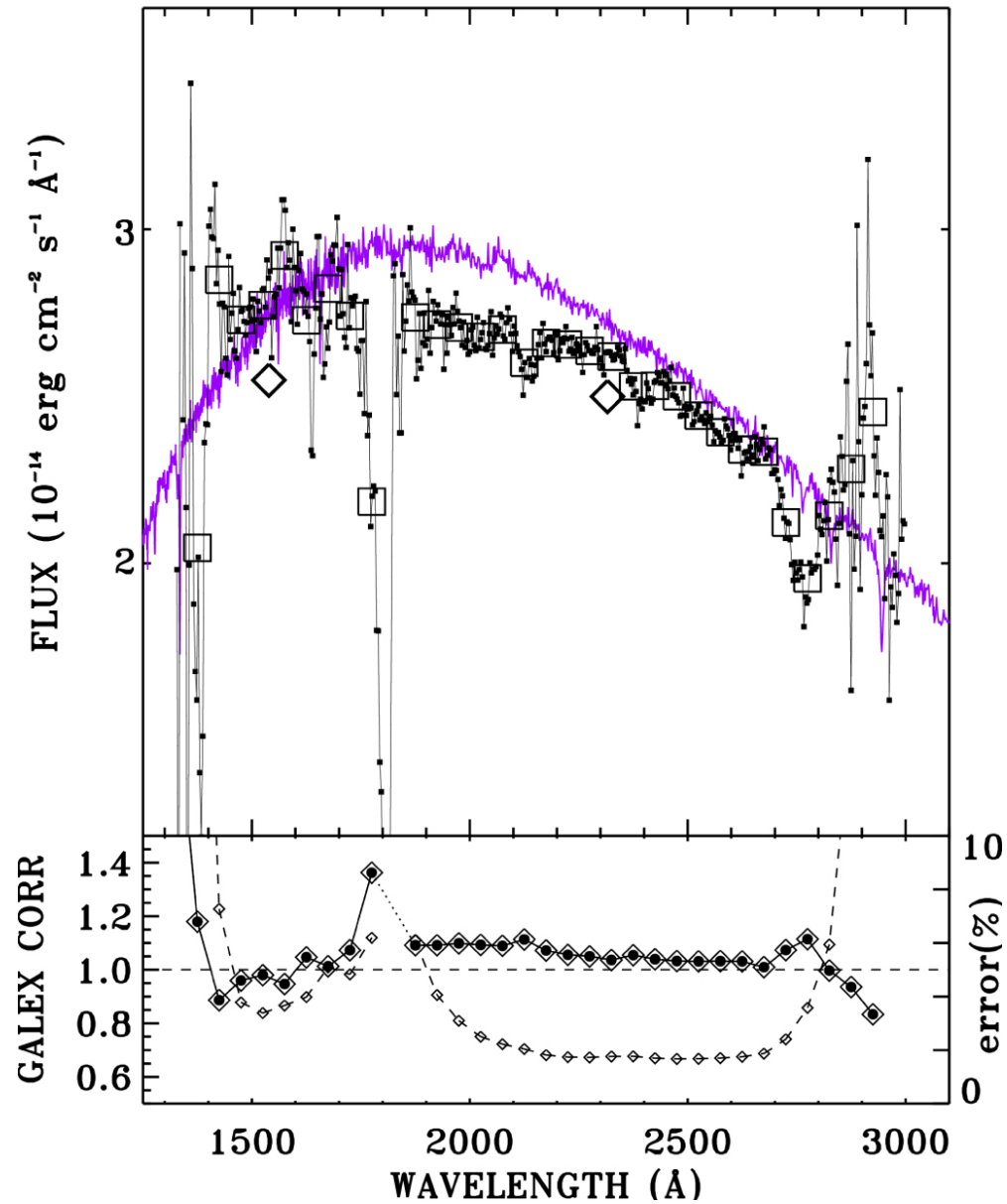
Figure 1. from A Correction for GALEX Spectroscopic UV Flux Distributions from Comparisons with CALSPEC and IUE null 2019 AJ 157 107 doi:10.3847/1538-3881/aafdb8 https://dx.doi.org/10.3847/1538-3881/aafdb8 © 2019. The American Astronomical Society. All rights reserved.
