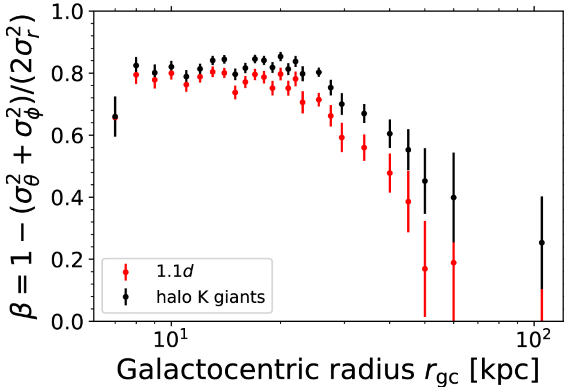
Figure 7. from Anisotropy of the Milky Way's Stellar Halo Using K Giants from LAMOST and Gaia null 2019 AJ 157 104 doi:10.3847/1538-3881/aafd2e https://dx.doi.org/10.3847/1538-3881/aafd2e © 2019. The American Astronomical Society. All rights reserved.
