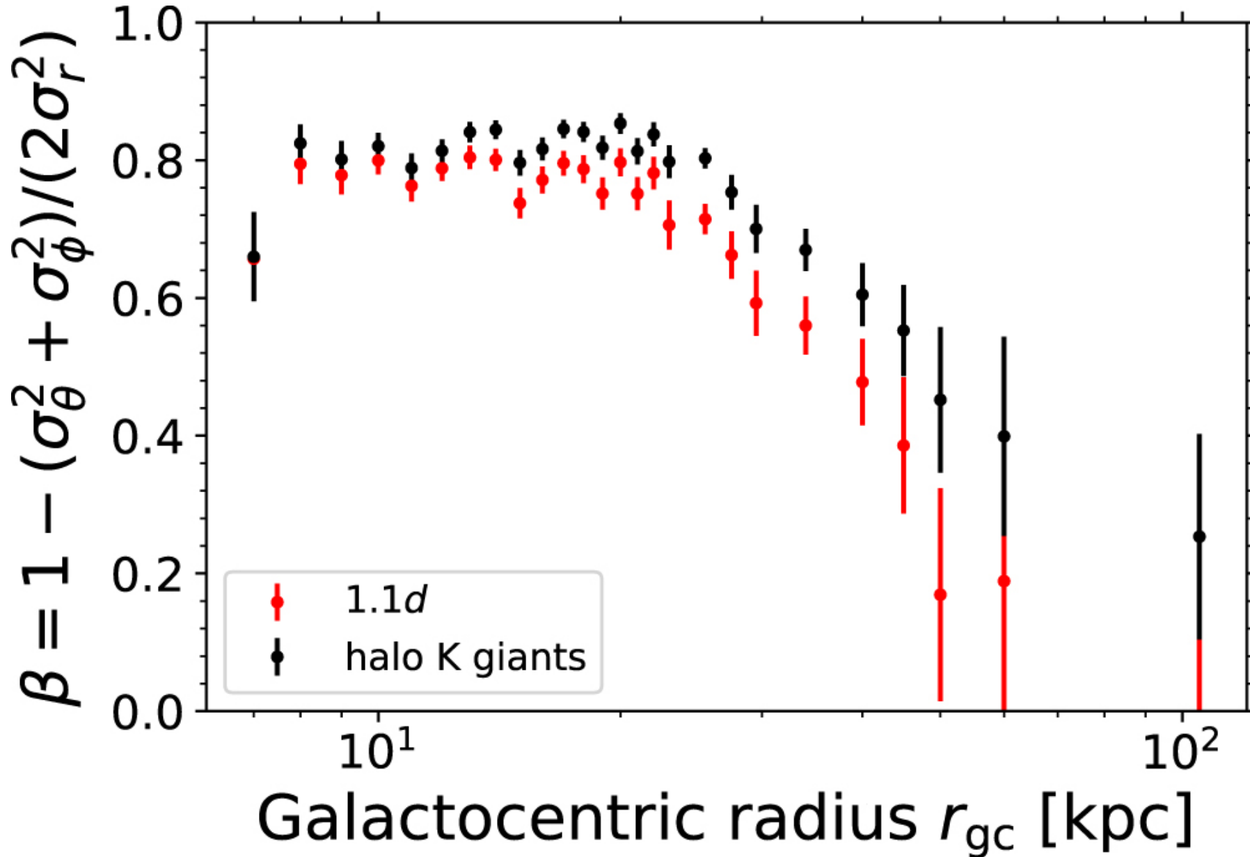
Figure 7. from Anisotropy of the Milky Way's Stellar Halo Using K Giants from LAMOST and Gaia null 2019 AJ 157 104 doi:10.3847/1538-3881/aafd2e http://dx.doi.org/10.3847/1538-3881/aafd2e © 2019. The American Astronomical Society. All rights reserved.
