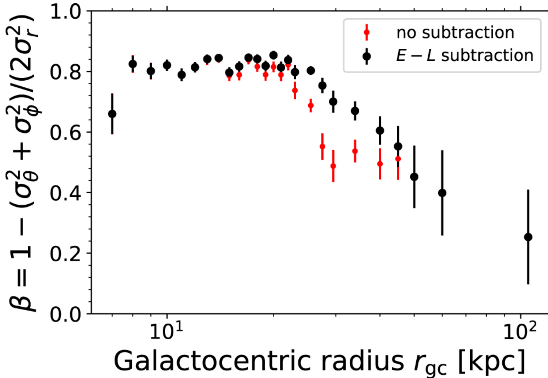
Figure 5. from Anisotropy of the Milky Way's Stellar Halo Using K Giants from LAMOST and Gaia null 2019 AJ 157 104 doi:10.3847/1538-3881/aafd2e https://dx.doi.org/10.3847/1538-3881/aafd2e © 2019. The American Astronomical Society. All rights reserved.
