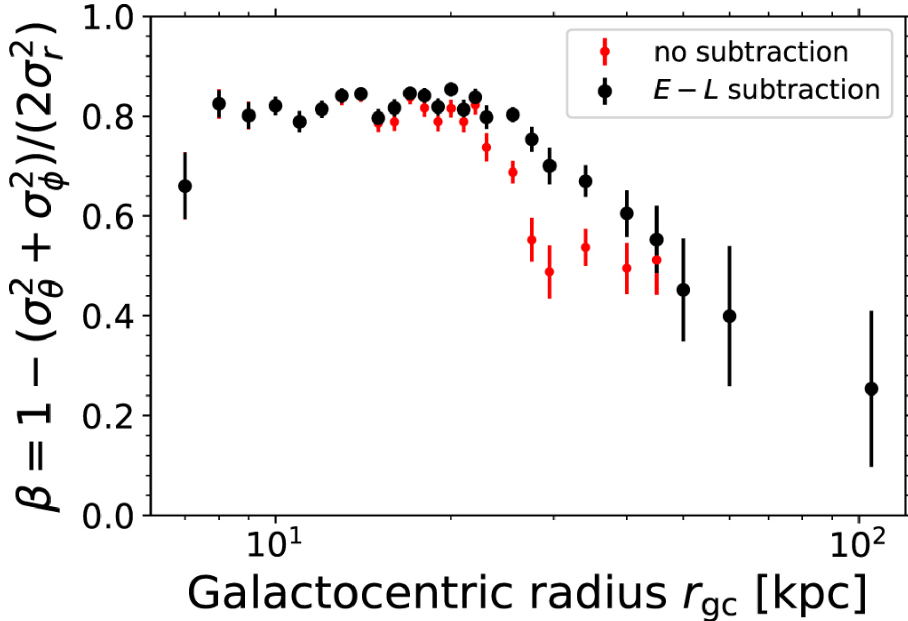
Figure 5. from Anisotropy of the Milky Way's Stellar Halo Using K Giants from LAMOST and Gaia null 2019 AJ 157 104 doi:10.3847/1538-3881/aafd2e http://dx.doi.org/10.3847/1538-3881/aafd2e © 2019. The American Astronomical Society. All rights reserved.
