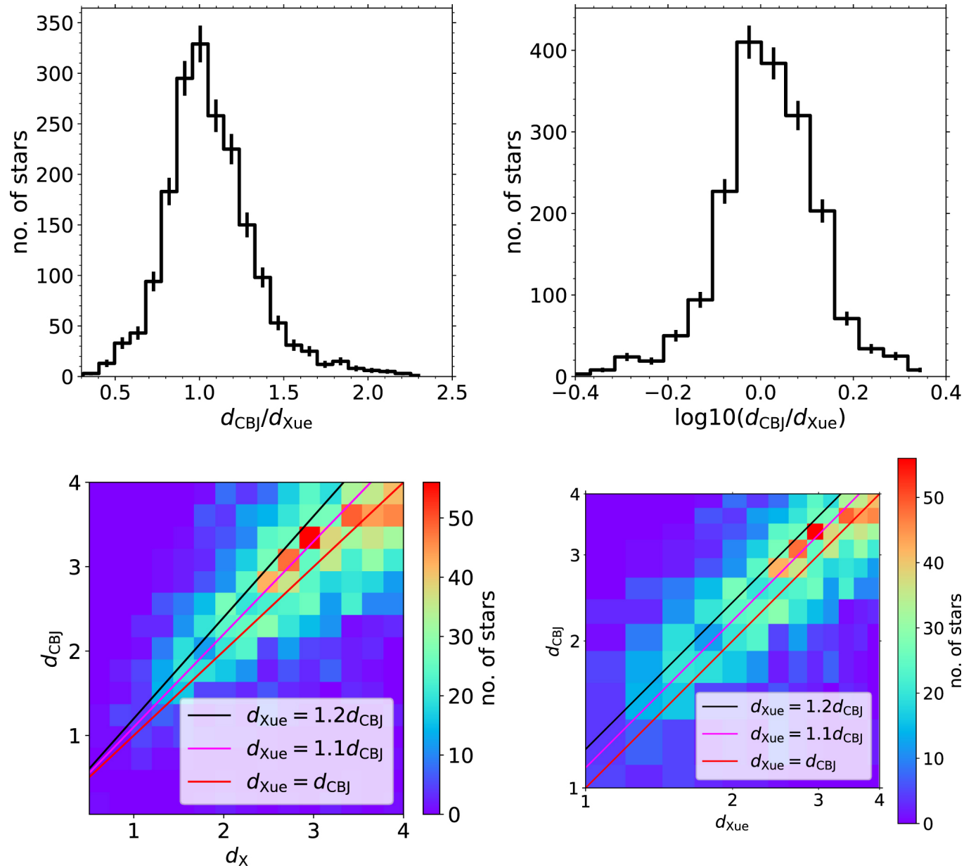
Figure 2. from Anisotropy of the Milky Way's Stellar Halo Using K Giants from LAMOST and Gaia null 2019 AJ 157 104 doi:10.3847/1538-3881/aafd2e https://dx.doi.org/10.3847/1538-3881/aafd2e © 2019. The American Astronomical Society. All rights reserved.
