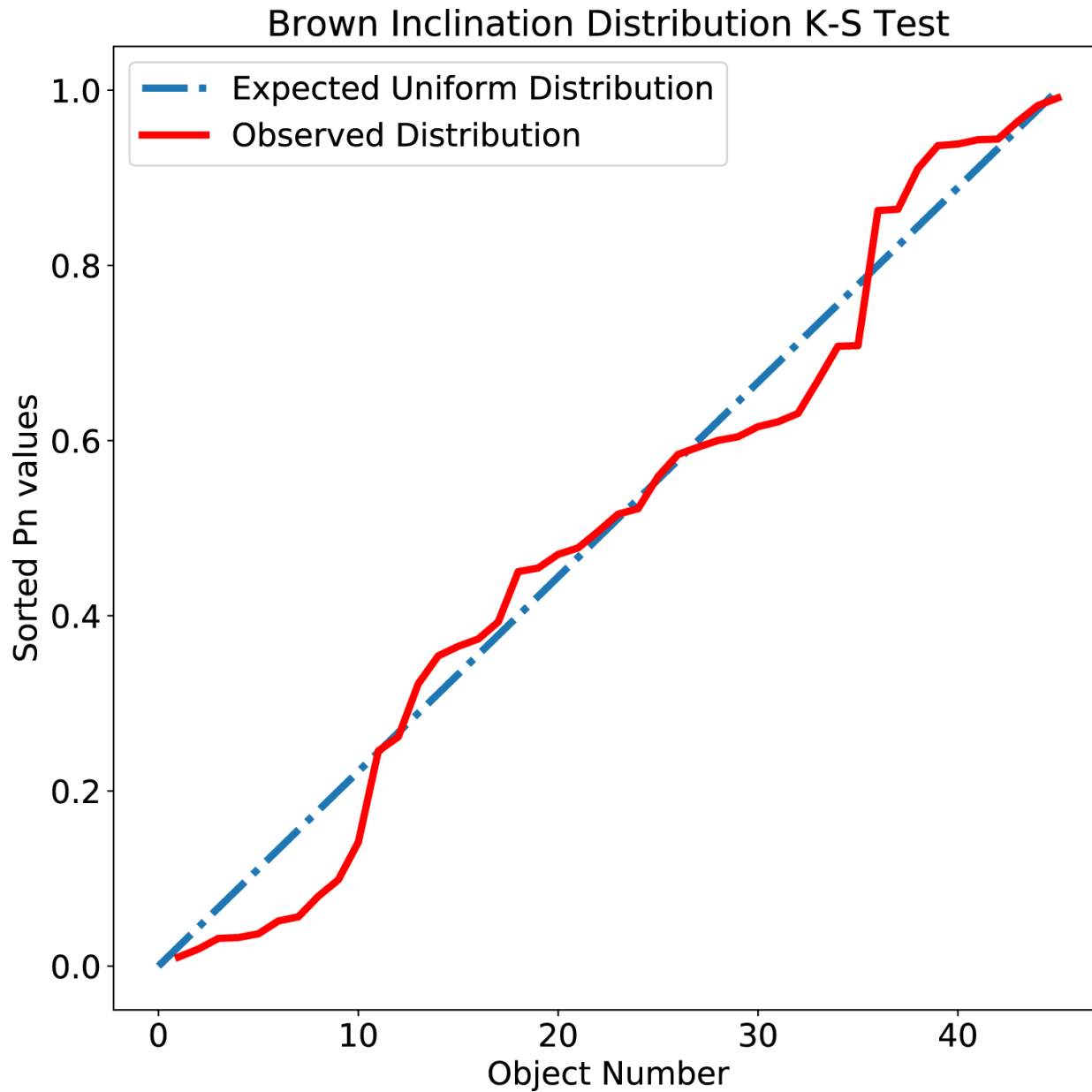
Figure 7. from Fast Algorithms for Slow Moving Asteroids: Constraints on the Distribution of Kuiper Belt Objects null 2019 AJ 157 119 doi:10.3847/1538-3881/aafd2d https://dx.doi.org/10.3847/1538-3881/aafd2d © 2019. The American Astronomical Society. All rights reserved.
