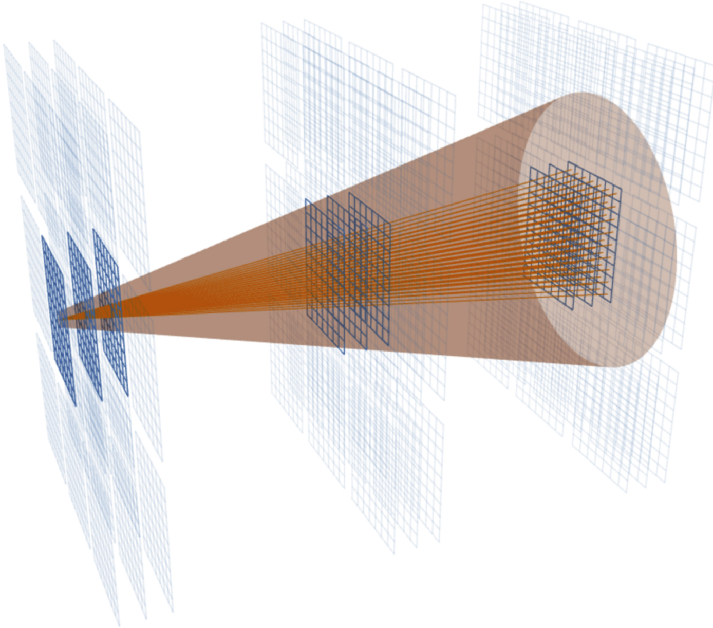
Figure 2. from Fast Algorithms for Slow Moving Asteroids: Constraints on the Distribution of Kuiper Belt Objects null 2019 AJ 157 119 doi:10.3847/1538-3881/aafd2d https://dx.doi.org/10.3847/1538-3881/aafd2d © 2019. The American Astronomical Society. All rights reserved.
