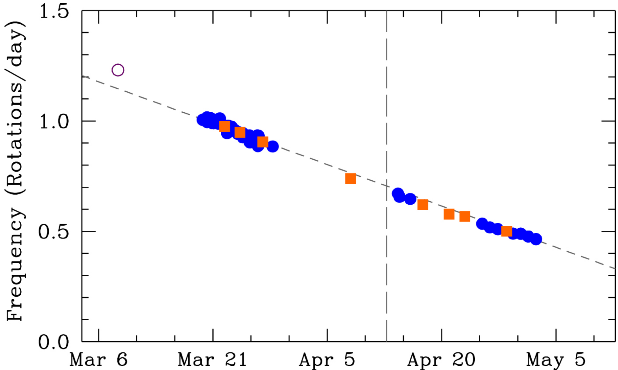
Figure 7. from Gas Jet Morphology and the Very Rapidly Increasing Rotation Period of Comet 41P/Tuttle–Giacobini–Kresák null 2019 AJ 157 108 doi:10.3847/1538-3881/aafbabb https://dx.doi.org/10.3847/1538-3881/aafbabb © 2019. The American Astronomical Society. All rights reserved.
