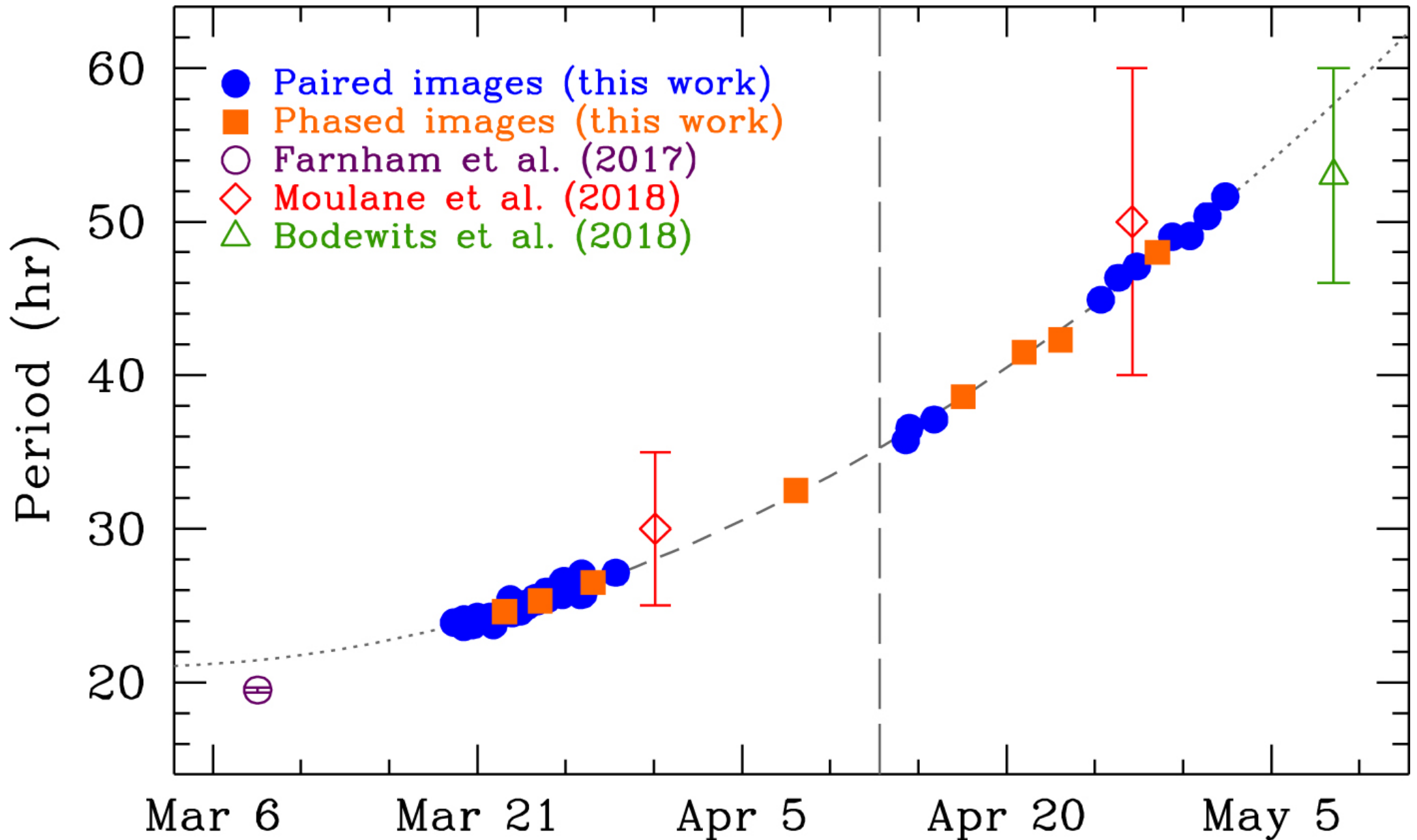
Figure 5. from Gas Jet Morphology and the Very Rapidly Increasing Rotation Period of Comet 41P/Tuttle–Giacobini–Kresák null 2019 AJ 157 108 doi:10.3847/1538-3881/aafbab https://dx.doi.org/10.3847/1538-3881/aafbab © 2019. The American Astronomical Society. All rights reserved.
