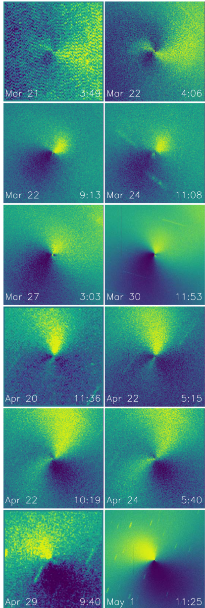
Figure 4. from Gas Jet Morphology and the Very Rapidly Increasing Rotation Period of Comet 41P/Tuttle–Giacobini–Kresák null 2019 AJ 157 108 doi:10.3847/1538-3881/aafbab https://dx.doi.org/10.3847/1538-3881/aafbab © 2019. The American Astronomical Society. All rights reserved.
