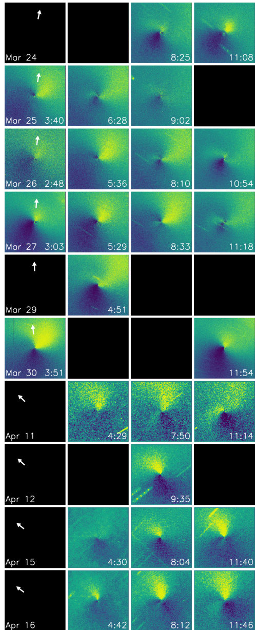
Figure 3. from Gas Jet Morphology and the Very Rapidly Increasing Rotation Period of Comet 41P/Tuttle–Giacobini–Kresák null 2019 AJ 157 108 doi:10.3847/1538-3881/aafbabb https://dx.doi.org/10.3847/1538-3881/aafbabb © 2019. The American Astronomical Society. All rights reserved.
