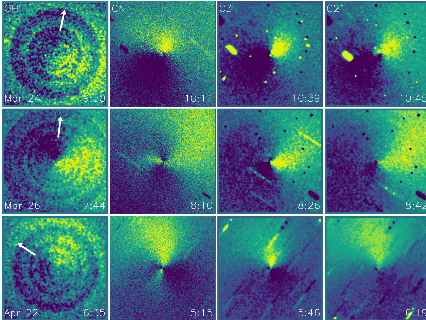
Figure 2. from Gas Jet Morphology and the Very Rapidly Increasing Rotation Period of Comet 41P/Tuttle–Giacobini–Kresák null 2019 AJ 157 108 doi:10.3847/1538-3881/aafbab https://dx.doi.org/10.3847/1538-3881/aafbab © 2019. The American Astronomical Society. All rights reserved.
