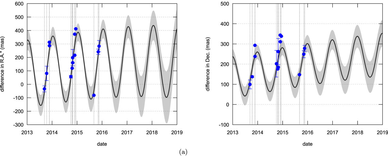
Figure 6. from Astrometry and Occultation Predictions to Trans-Neptunian and Centaur Objects Observed within the Dark Energy Survey null 2019 AJ 157 120 doi:10.3847/1538-3881/aafb37 https://dx.doi.org/10.3847/1538-3881/aafb37 © 2019. The American Astronomical Society. All rights reserved.
