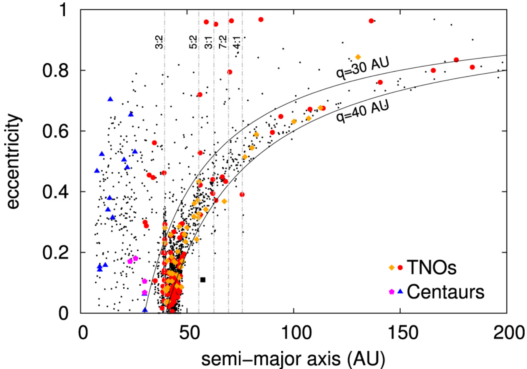
Figure 5. from Astrometry and Occultation Predictions to Trans-Neptunian and Centaur Objects Observed within the Dark Energy Survey null 2019 AJ 157 120 doi:10.3847/1538-3881/aafb37 https://dx.doi.org/10.3847/1538-3881/aafb37 © 2019. The American Astronomical Society. All rights reserved.
