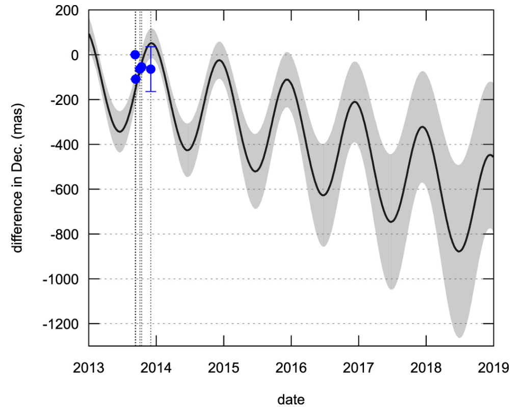
Figure 2. from Astrometry and Occultation Predictions to Trans-Neptunian and Centaur Objects Observed within the Dark Energy Survey null 2019 AJ 157 120 doi:10.3847/1538-3881/aafb37 https://dx.doi.org/10.3847/1538-3881/aafb37 © 2019. The American Astronomical Society. All rights reserved.
