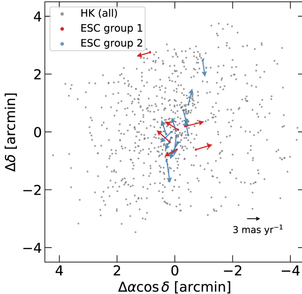
Figure 7. from Stellar Proper Motions in the Orion Nebula Cluster null 2019 AJ 157 109 doi:10.3847/1538-3881/aafb09 https://dx.doi.org/10.3847/1538-3881/aafb09 © 2019. The American Astronomical Society. All rights reserved.
