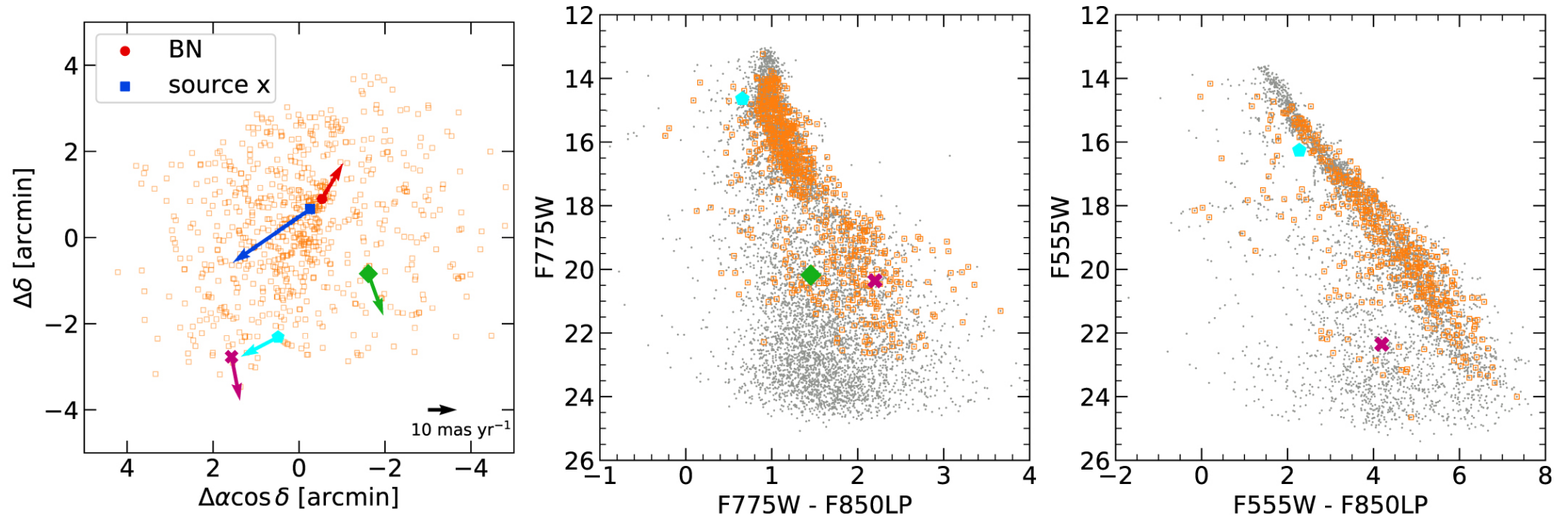
Figure 5. from Stellar Proper Motions in the Orion Nebula Cluster null 2019 AJ 157 109 doi:10.3847/1538-3881/aafb09 https://dx.doi.org/10.3847/1538-3881/aafb09 © 2019. The American Astronomical Society. All rights reserved.
