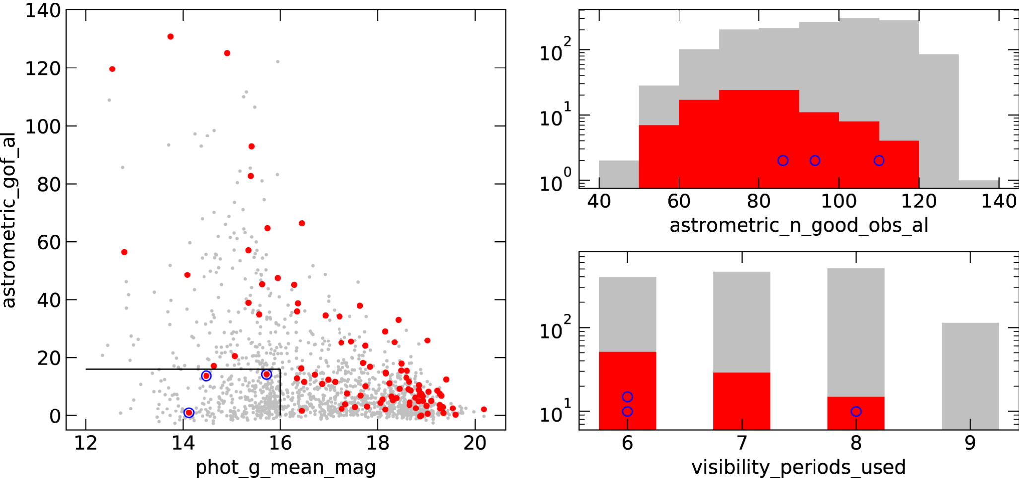
Figure 11. from Stellar Proper Motions in the Orion Nebula Cluster null 2019 AJ 157 109 doi:10.3847/1538-3881/aafb09 https://dx.doi.org/10.3847/1538-3881/aafb09 © 2019. The American Astronomical Society. All rights reserved.
